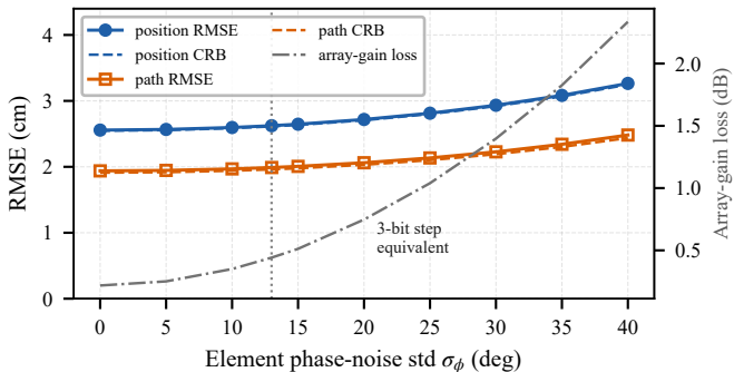
(a) Static element phase noise (3-bit R-RIS)
