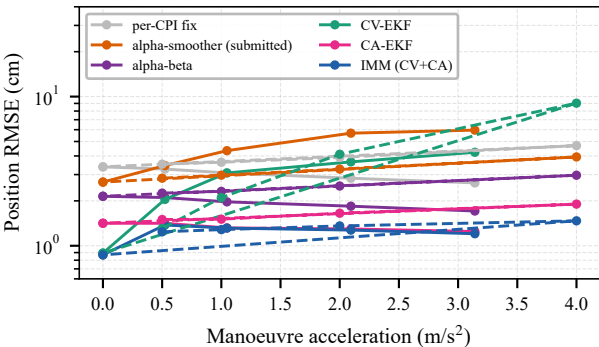
(b) Solid: coordinated turns; dashed: along-track acceleration
