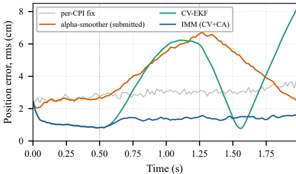
(a) S-manoeuvre: error versus time (dotted: turn reversals)
