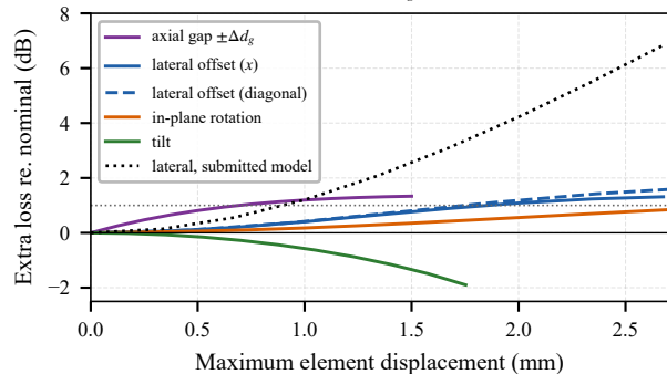
(b) Assembly errors at d_g = 2 mm, f=0.50
