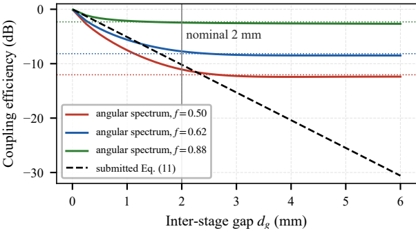
(a) Coupling versus gap (dotted: fundamental-mode limit f^4 )
