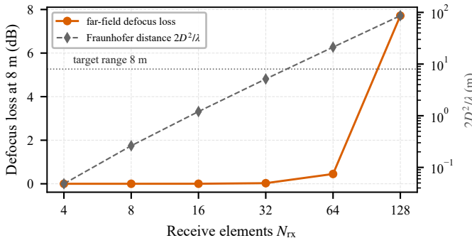
(b) Wavefront curvature of large receive arrays
