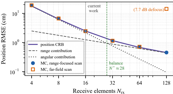
(a) Position accuracy versus receive aperture ( \beta = 60^\circ )
