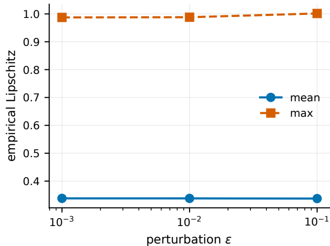
Empirical stability bound
