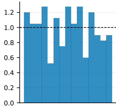
SBC ranks: gaussian linear
