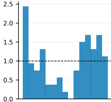
SBC ranks: two moons
