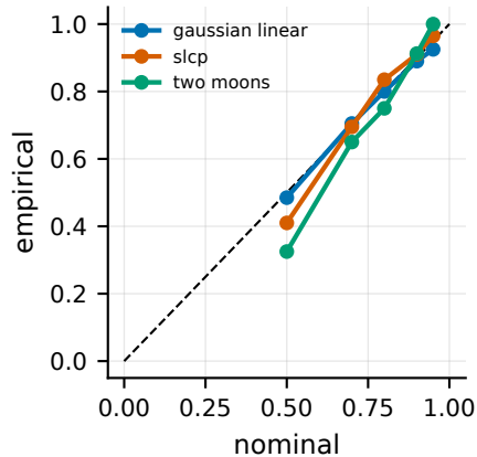
Reliability
