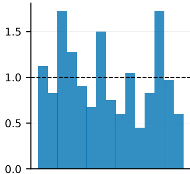
SBC ranks: slcp
