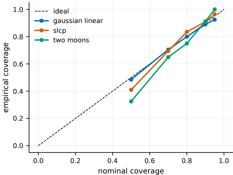
Coverage vs nominal
