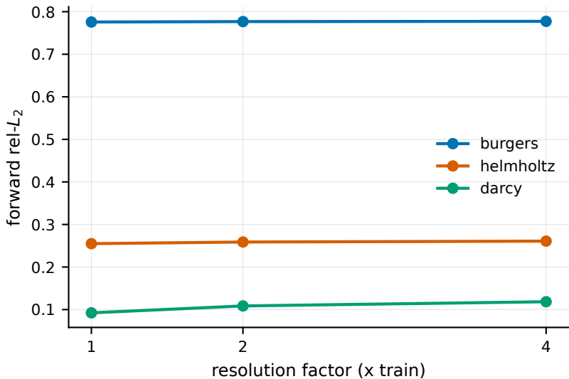
Zero-shot super-resolution
