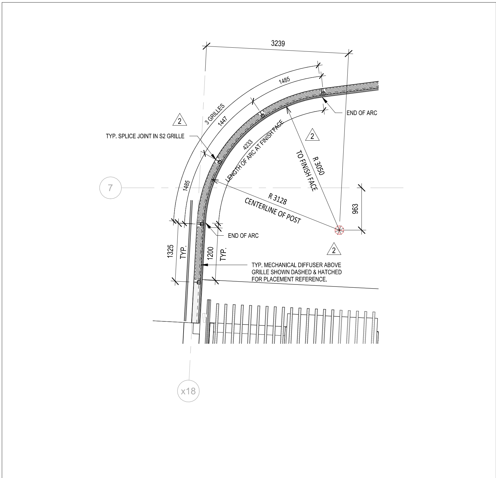
3 LEVEL 02 RCP - CEILING GRILLES - 3 A9.142 1:50
