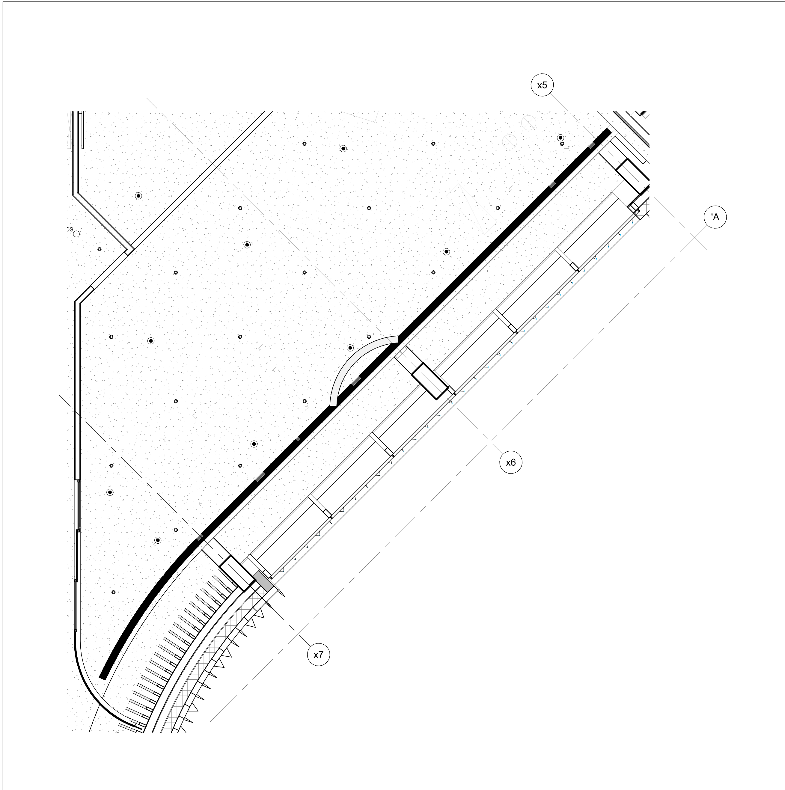
4 LEVEL 02 RCP - CEILING GRILLES - 4 A9.142 1:50
