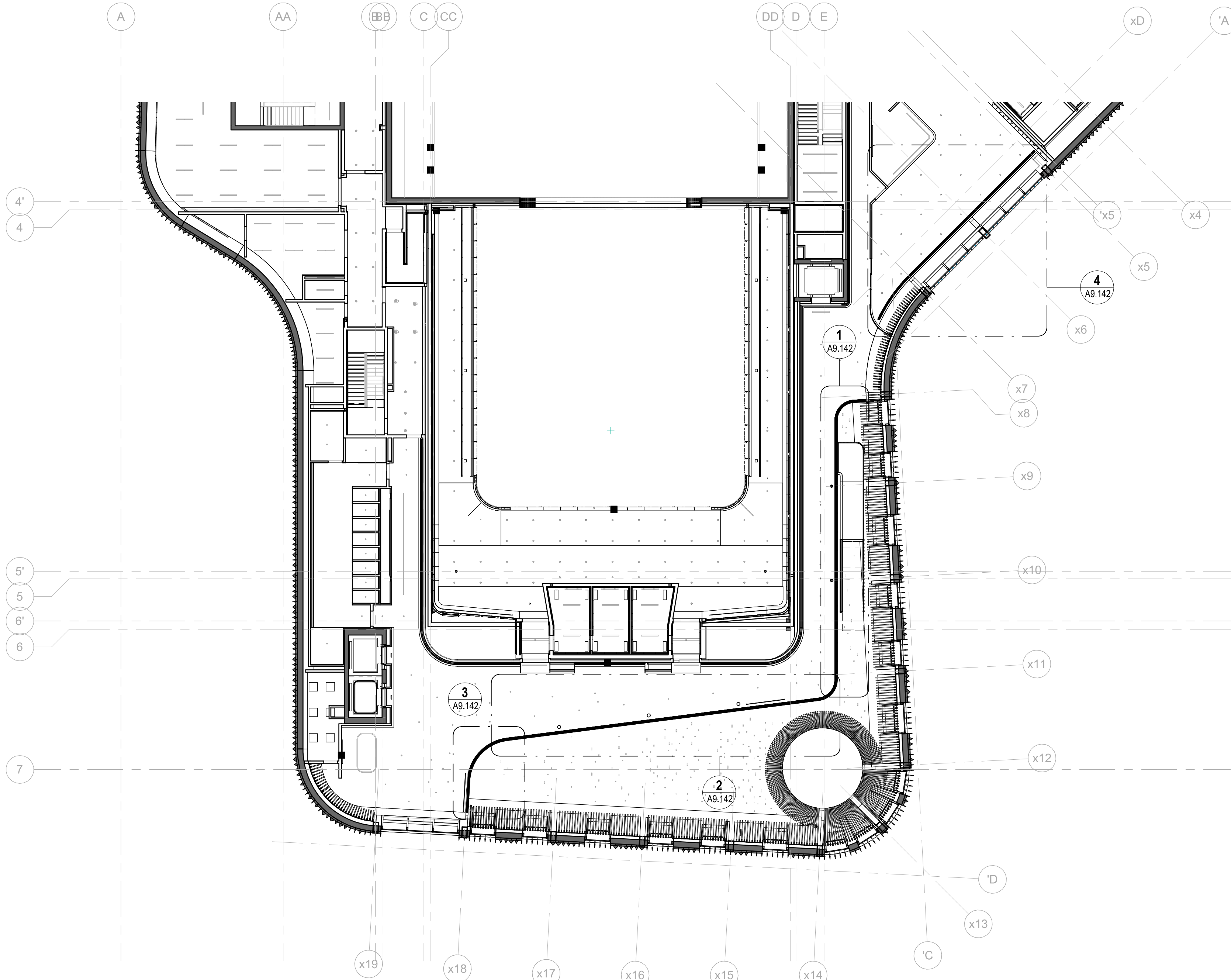
5 LEVEL 02 RCP - CEILING GRILLES A9.142 1:200
