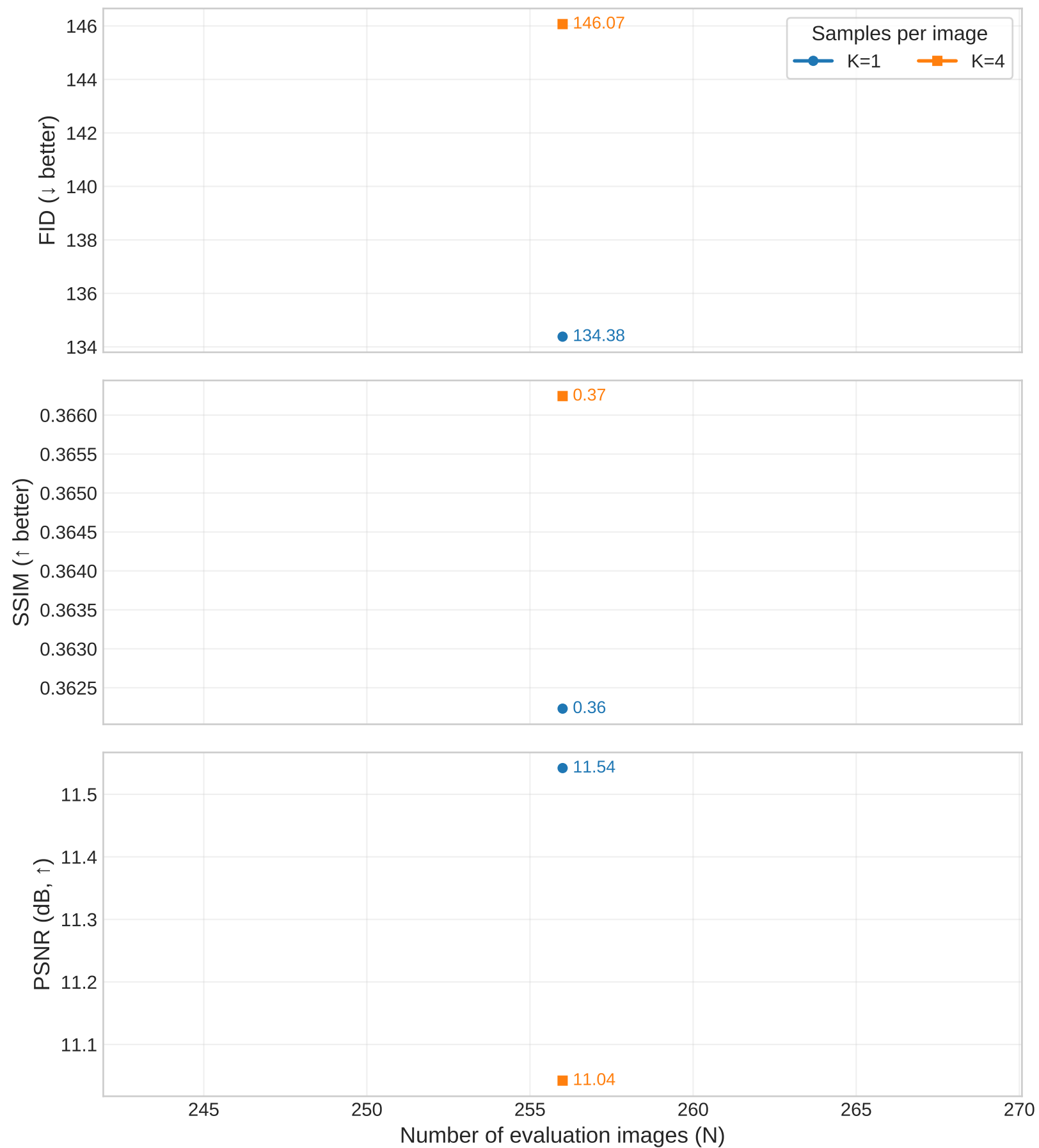
VAEAC Inpainting Metrics vs. Dataset Size — all
