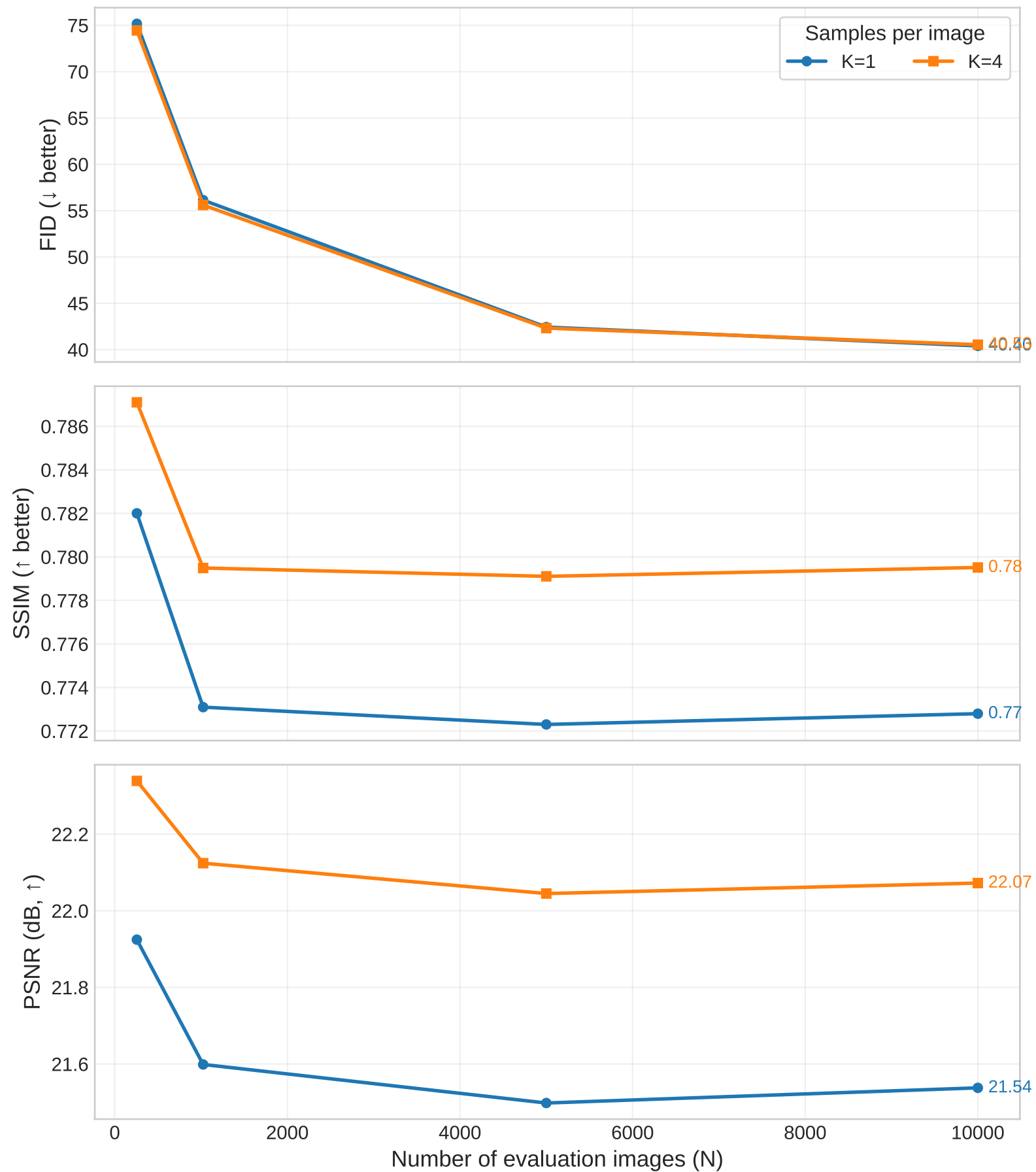
Inpainting Metrics vs. Dataset Size — celeba_train
