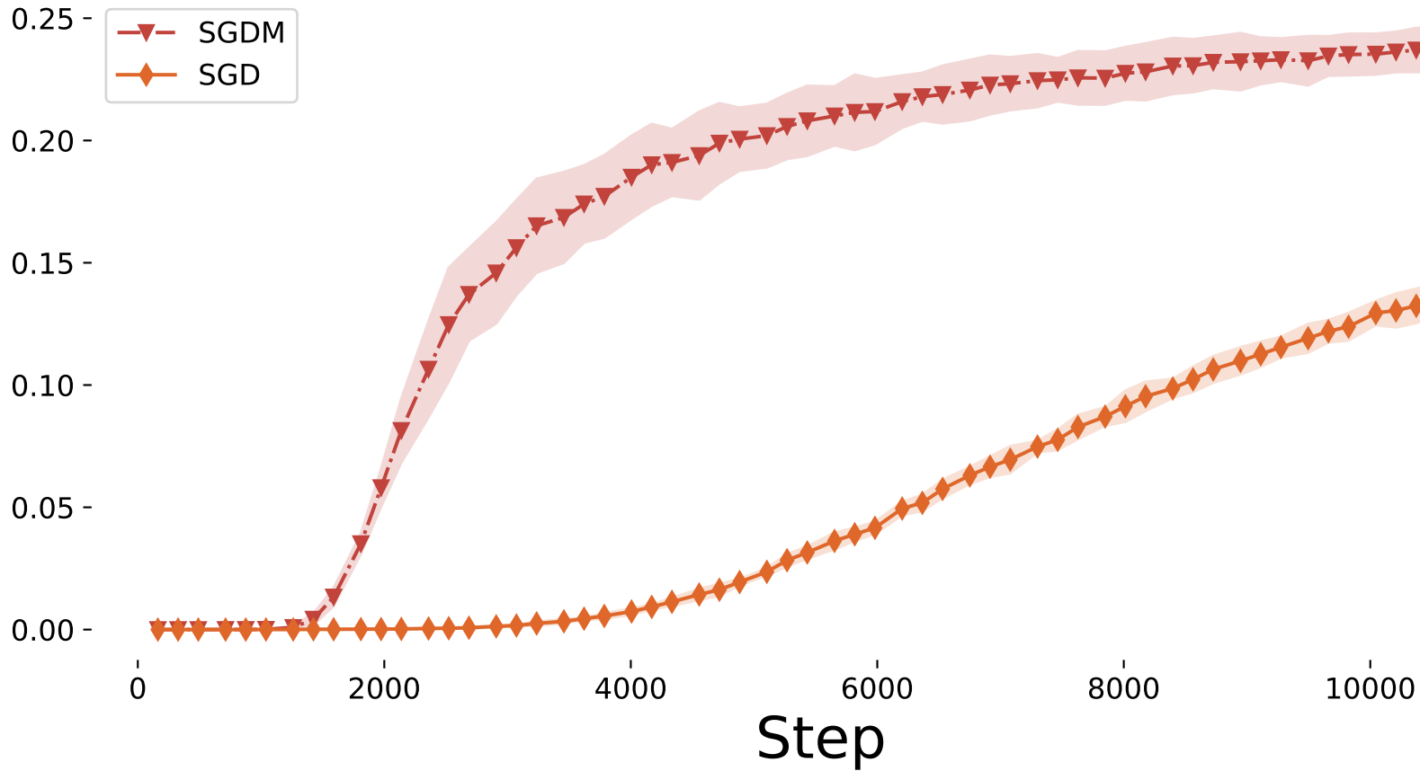
ROUGE-1
