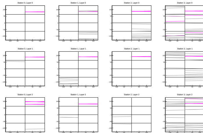
Figure: SCT Hits from Event 2840829, Run 022300. Note that out of time HITS (!01X) are shown in grey.
