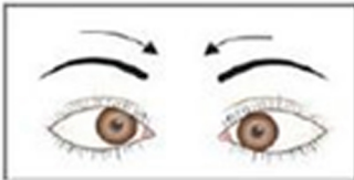
Convergence exercises
