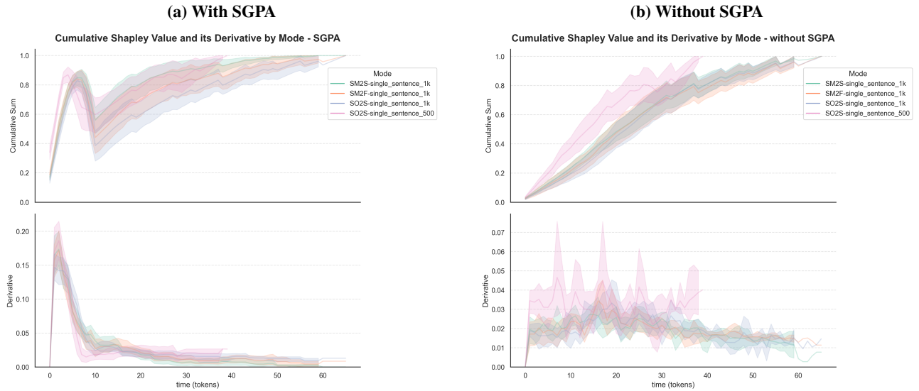
Figure 5: Position-normalized cumulative SV profile (with derivative) for speech-to-speech mode. Both conditions exhibit an “early mass” pattern, illustrating preserved macro-trend structure under SGPA.
