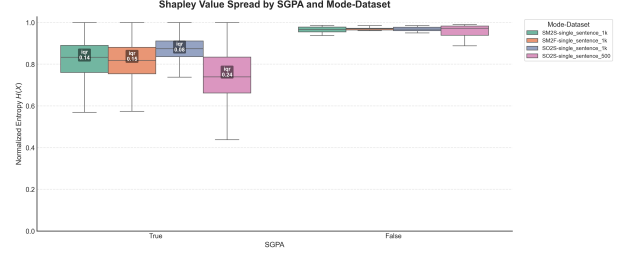
Figure 3: Normalized attribution entropy ( H/\sqrt{n} ) by mode with and without SGPA. SGPA widens the interquartile range, reflecting greater variability in concentration across samples.
