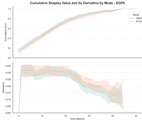
Figure 5: Position-normalized cumulative SV profile (with derivative) for speech-to-speech mode, illustrating the preserved “early mass” macro-trend under SGPA.
