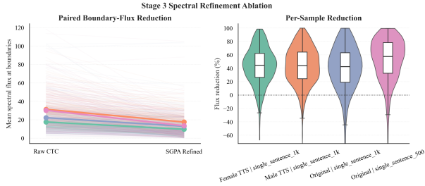
Figure 4: Stage 3 ablation overview. Left: per-sample paired flux before/after refinement; right: percent-reduction distribution.
