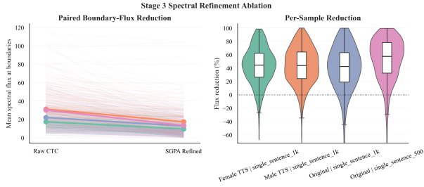
Figure 4: Stage 3 ablation overview. Left: per-sample paired flux before/after refinement; right: percent-reduction distribution.
