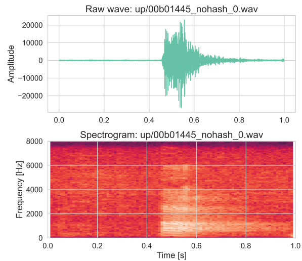
Figure 15: Raw wave and spectrogram example from train set for "up".
