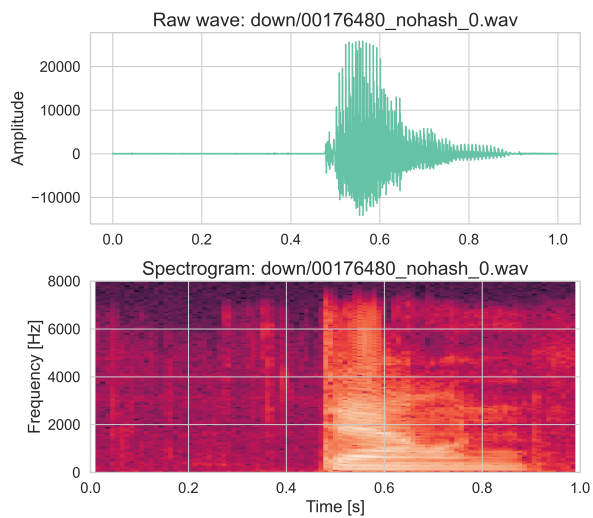
Figure 13: Raw wave and spectrogram example from train set for "down".
