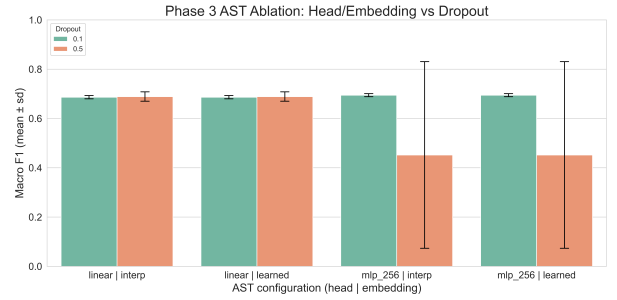
Figure 9: Phase 3 results: Ablation study for AST.
