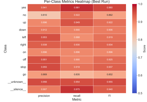
Figure 12: Phase 4 results: Per-class performance for the best performing model.
