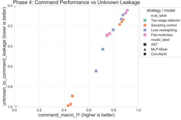
Figure 10: Phase 4 results: Command scores vs. Non-command scores for different strategies.
