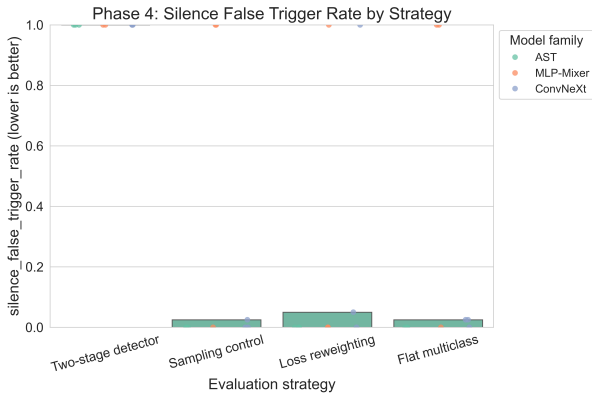
Figure 11: Phase 4 results: Silence false trigger rates for different strategies.
