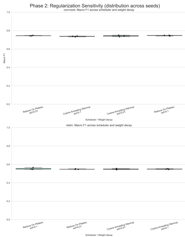
Figure 16: Regularization sensitivity across different configurations.
