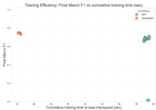
Figure 18: Training efficiency for different strategies.
