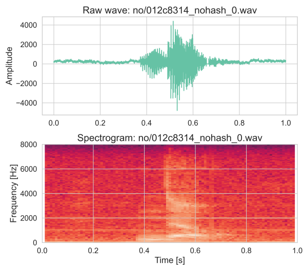
Figure 14: Raw wave and spectrogram example from train set for "no".
