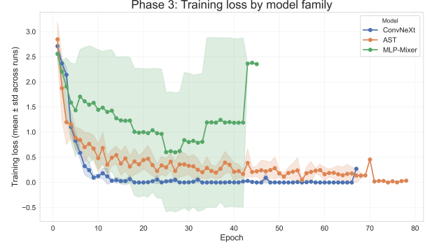
Figure 8: Phase 3 results: Training loss vs. epoch for different model families.
