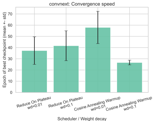
Phase 2: Epoch to Best Validation Result
