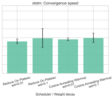
Phase 2: Epoch to Best Validation Result
