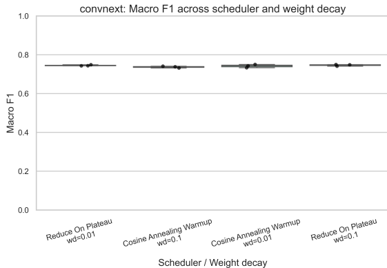
Phase 2: Regularization Sensitivity (distribution across seeds)
