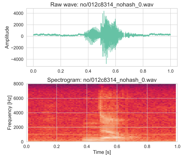
Figure 12: Raw wave and spectrogram example from train set for "no".
