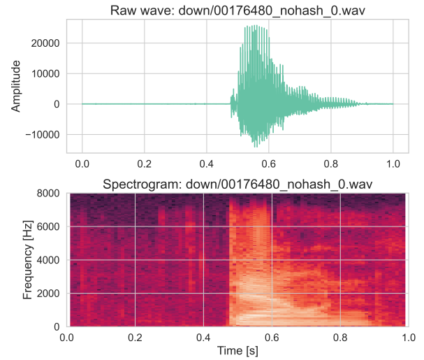
Figure 11: Raw wave and spectrogram example from train set for "down".
