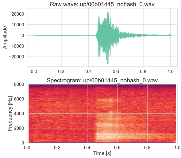
Figure 13: Raw wave and spectrogram example from train set for "up".
