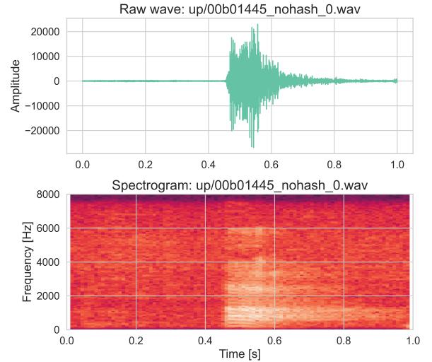
Figure 6: Raw wave and spectrogram example from train set for “up”.
