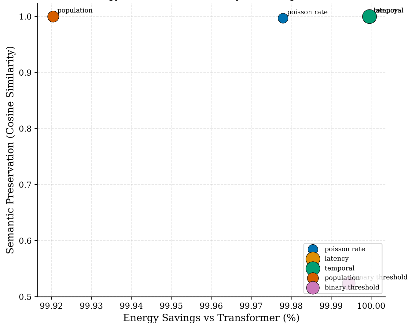
Energy-Semantic Tradeoff by Encoding Method
