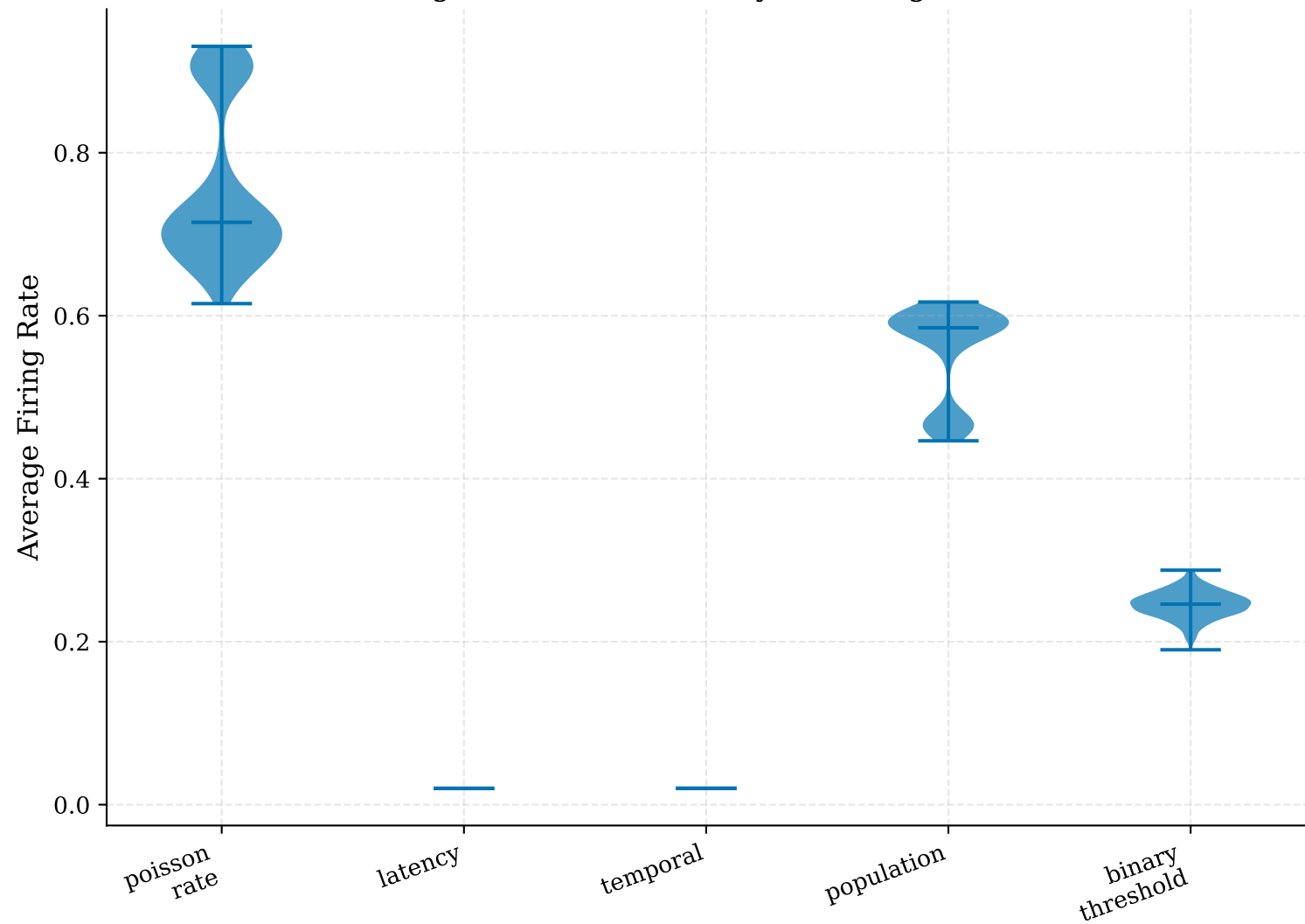
Firing Rate Distribution by Encoding Method
