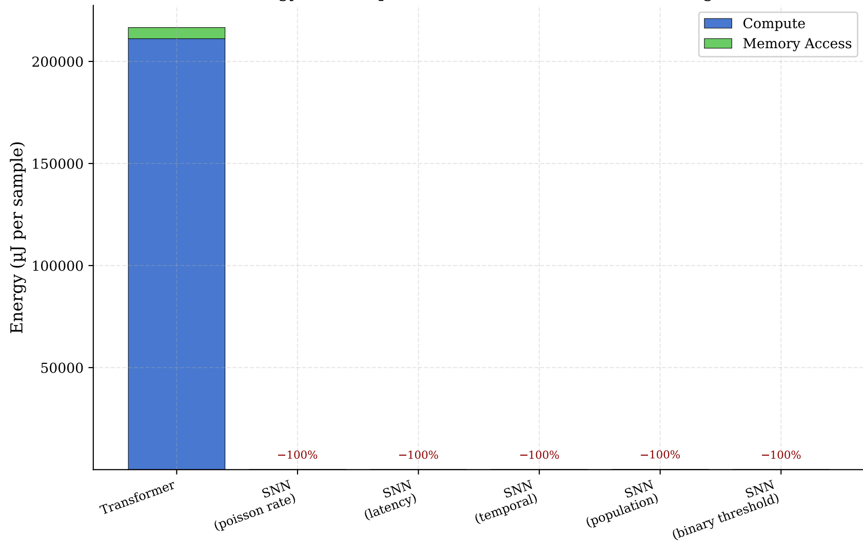
Energy Consumption: Transformer vs SNN Encodings
