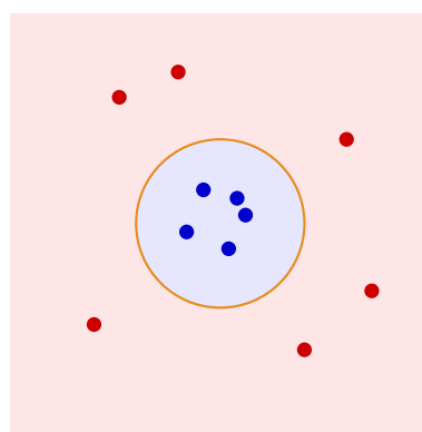
32 neurons — curved boundary
