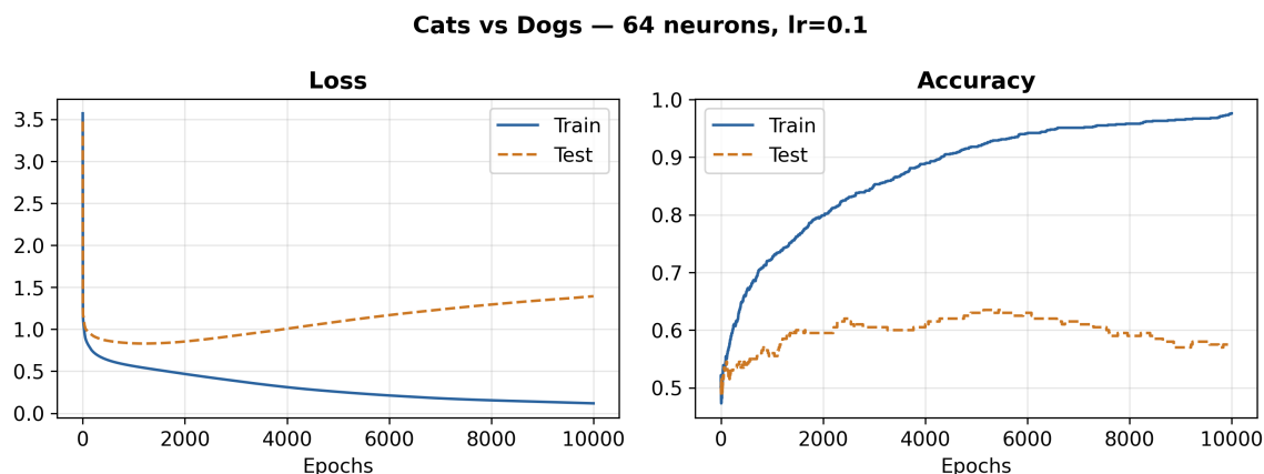
Figure 9: Train vs test performance on cats vs dogs. The training curves look great — but the test curves tell a different story. This is overfitting .
