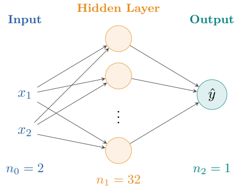
Figure 2: Architecture of our two-layer neural network: 2 inputs, 32 hidden neurons, 1 output.
