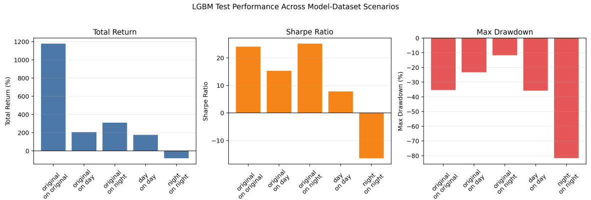
Figure 4: LGBM test performance by scenario. The original model generalizes better than the night-specific model in this experiment.
