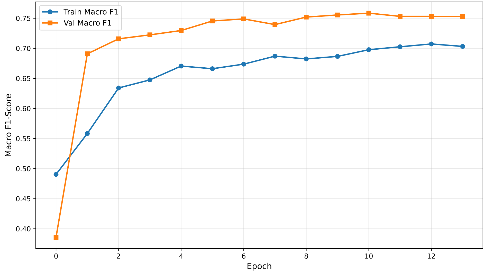
Training and Validation Macro F1-Score
