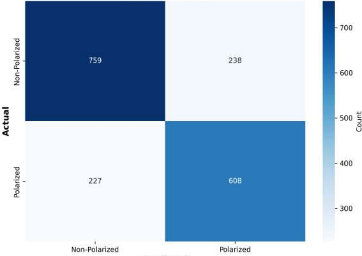
Confusion Matrix
