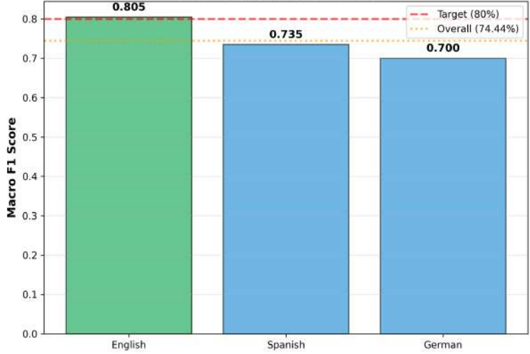
Per-Language Performance
