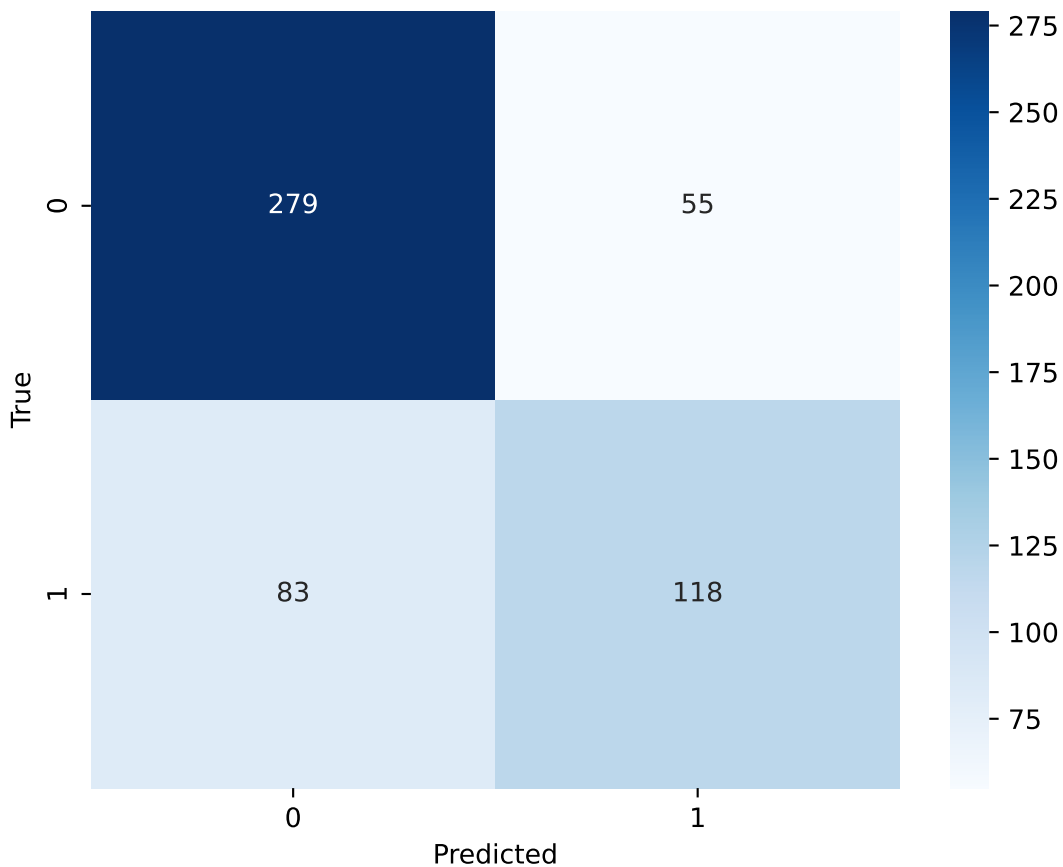
Random Forest — Confusion Matrix (ENG)
