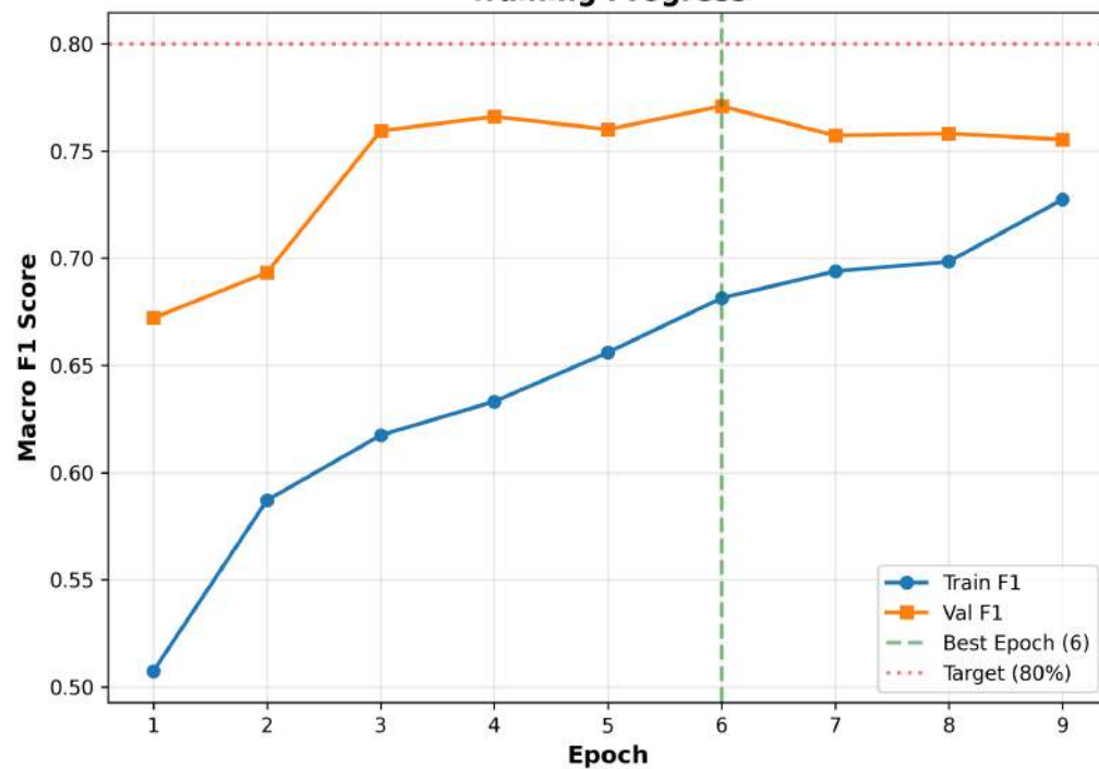
Training Progress
