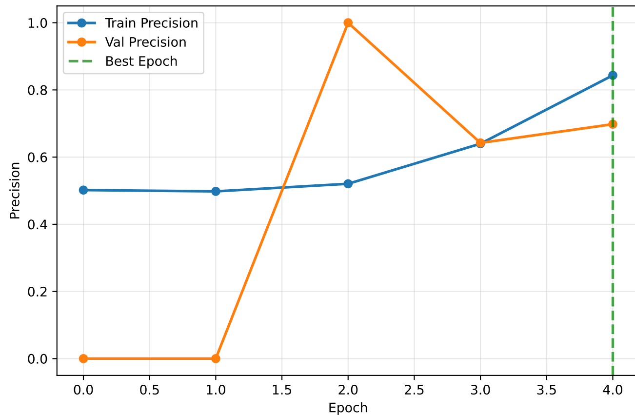
Model Precision
