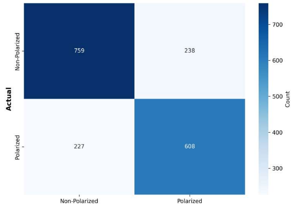
Confusion Matrix
