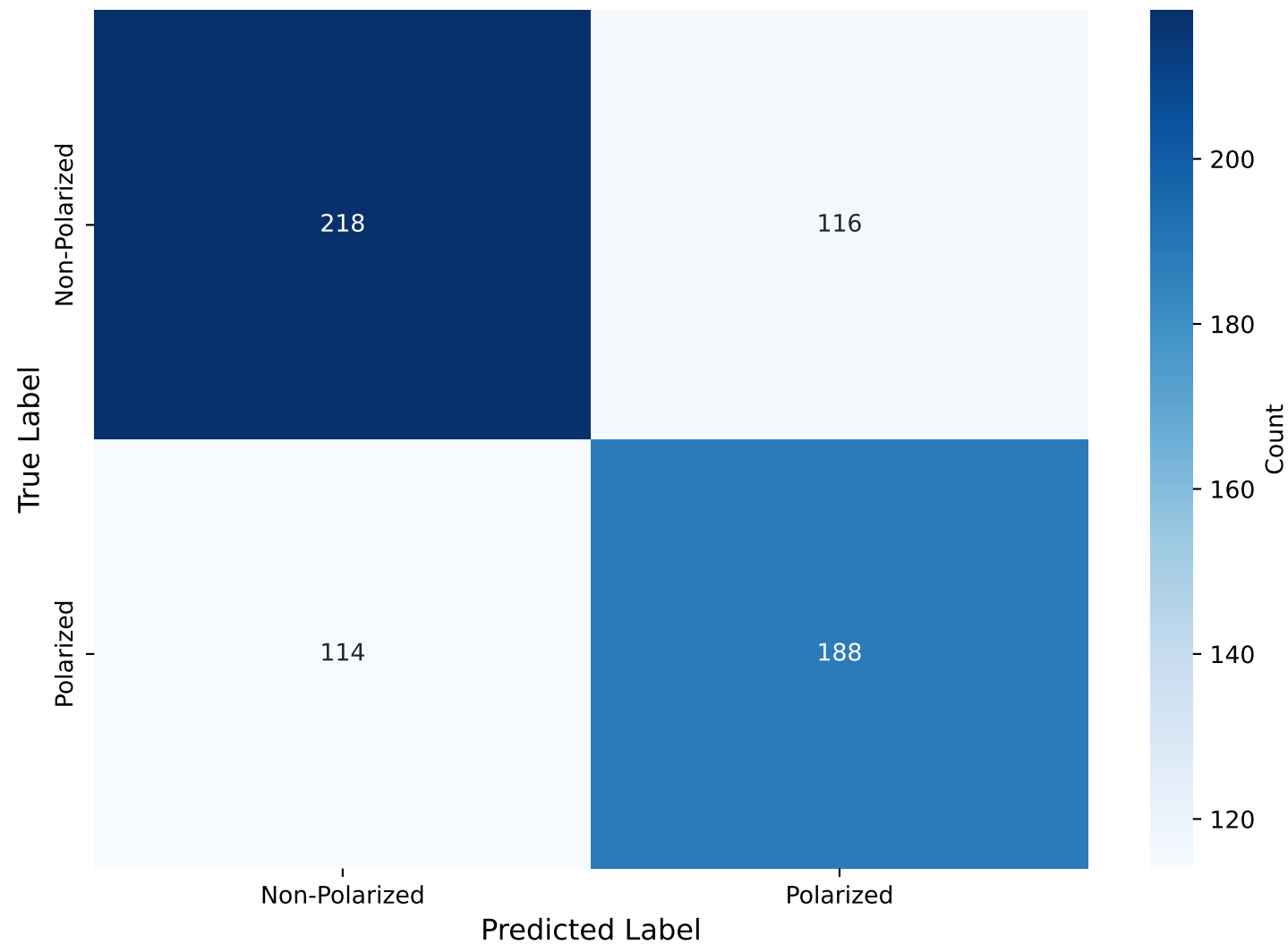
Confusion Matrix - German
