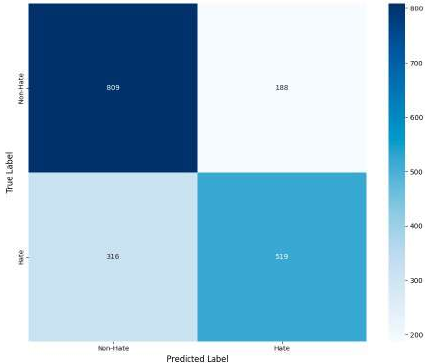
Confusion Matrix - XLM-RoBERTa-Base
