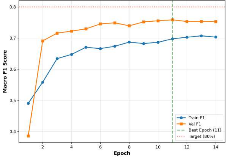
Training Progress
