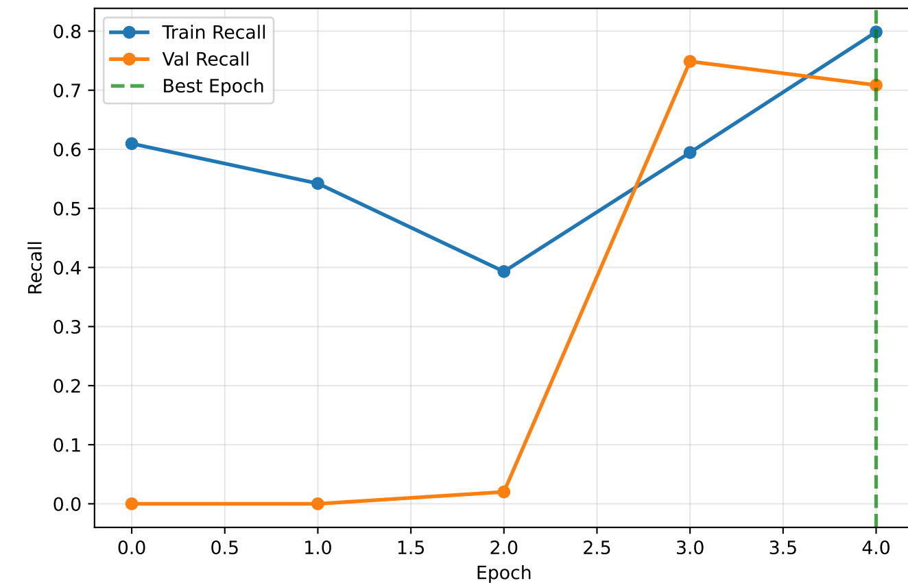
Model Recall
