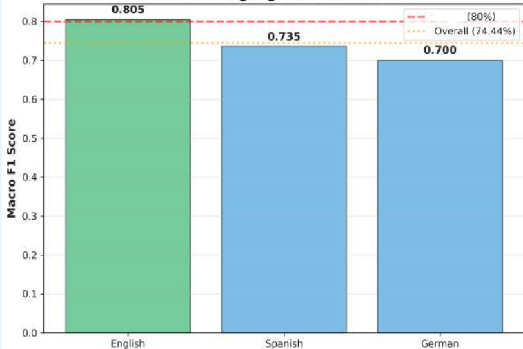
Per-Language Performance
