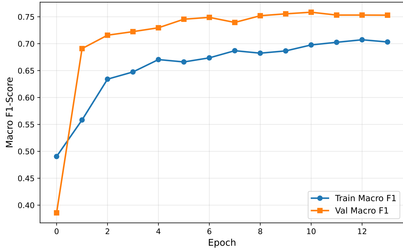
Training and Validation Macro F1-Score
