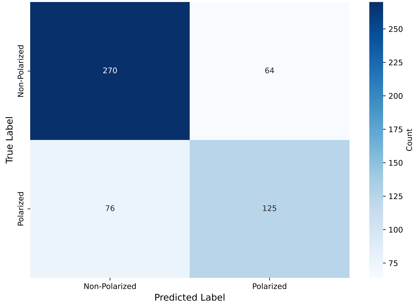
Confusion Matrix - English
