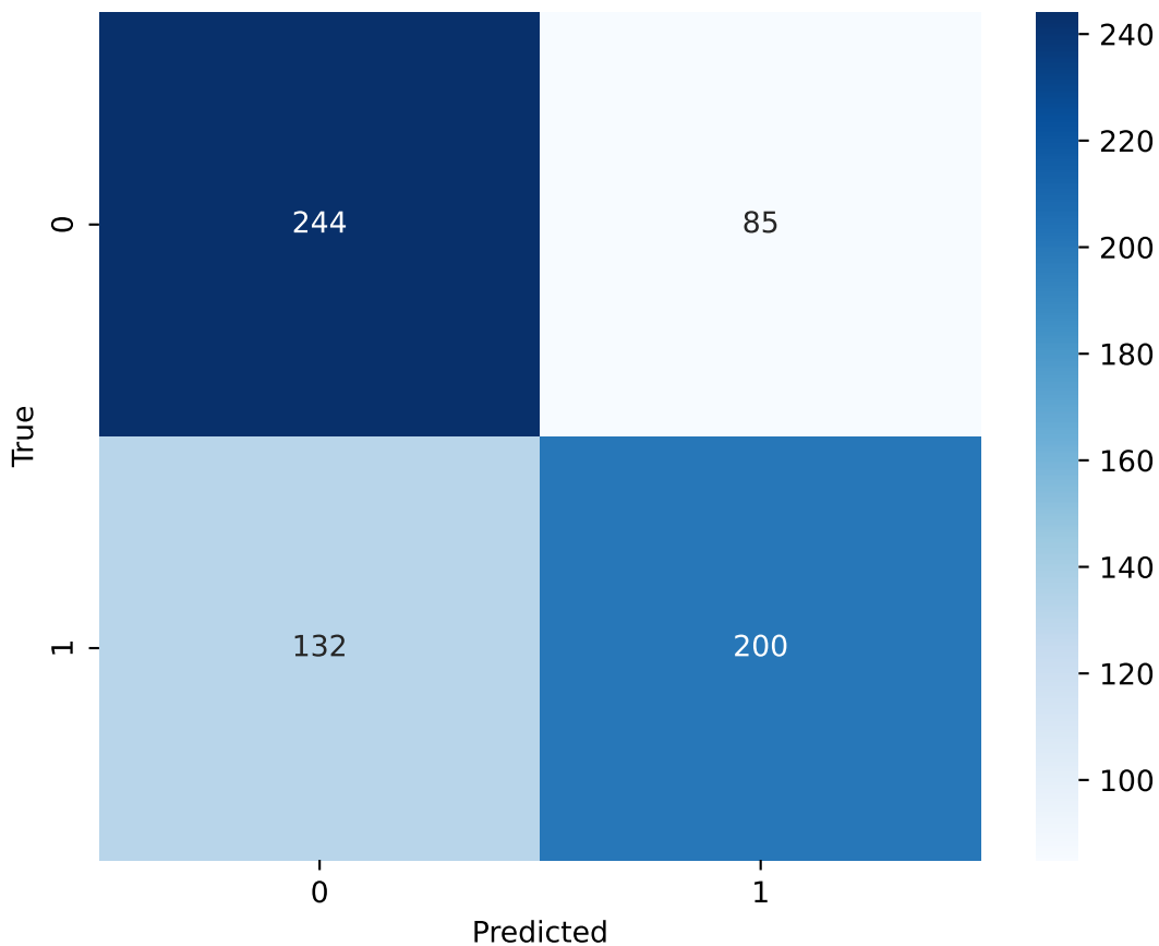
Random Forest — Confusion Matrix (SPA)
