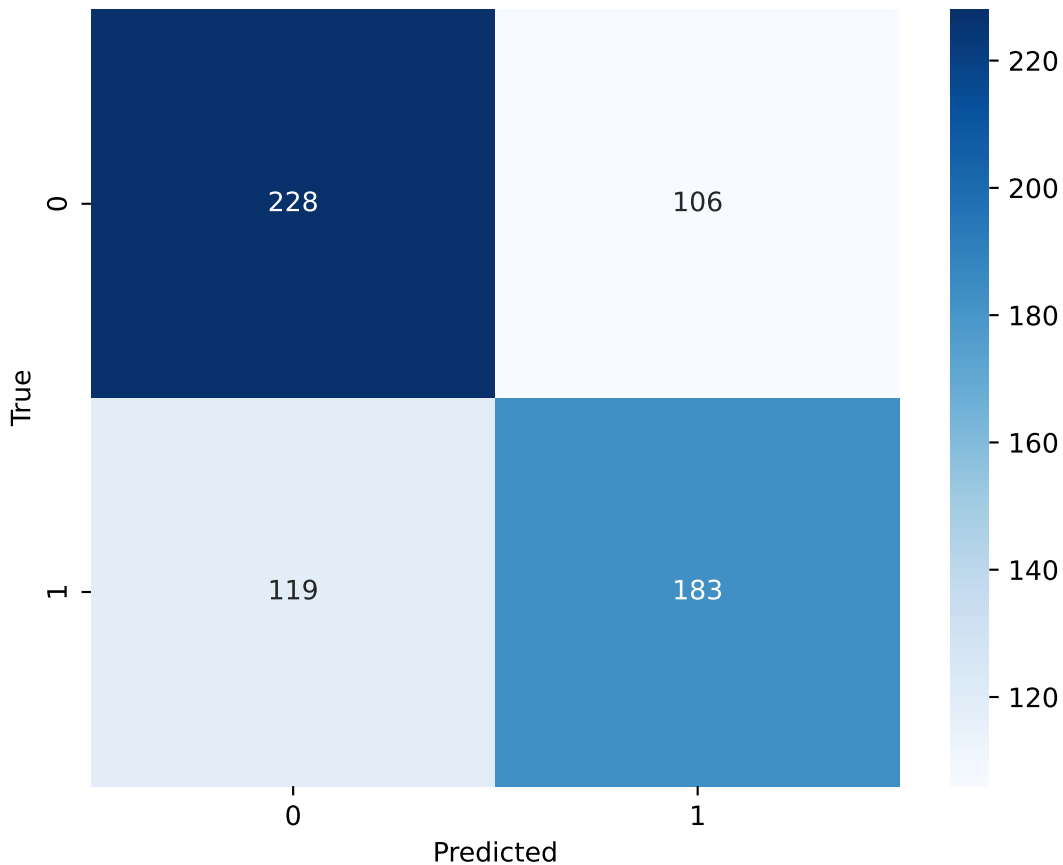
Random Forest — Confusion Matrix (DEU)
