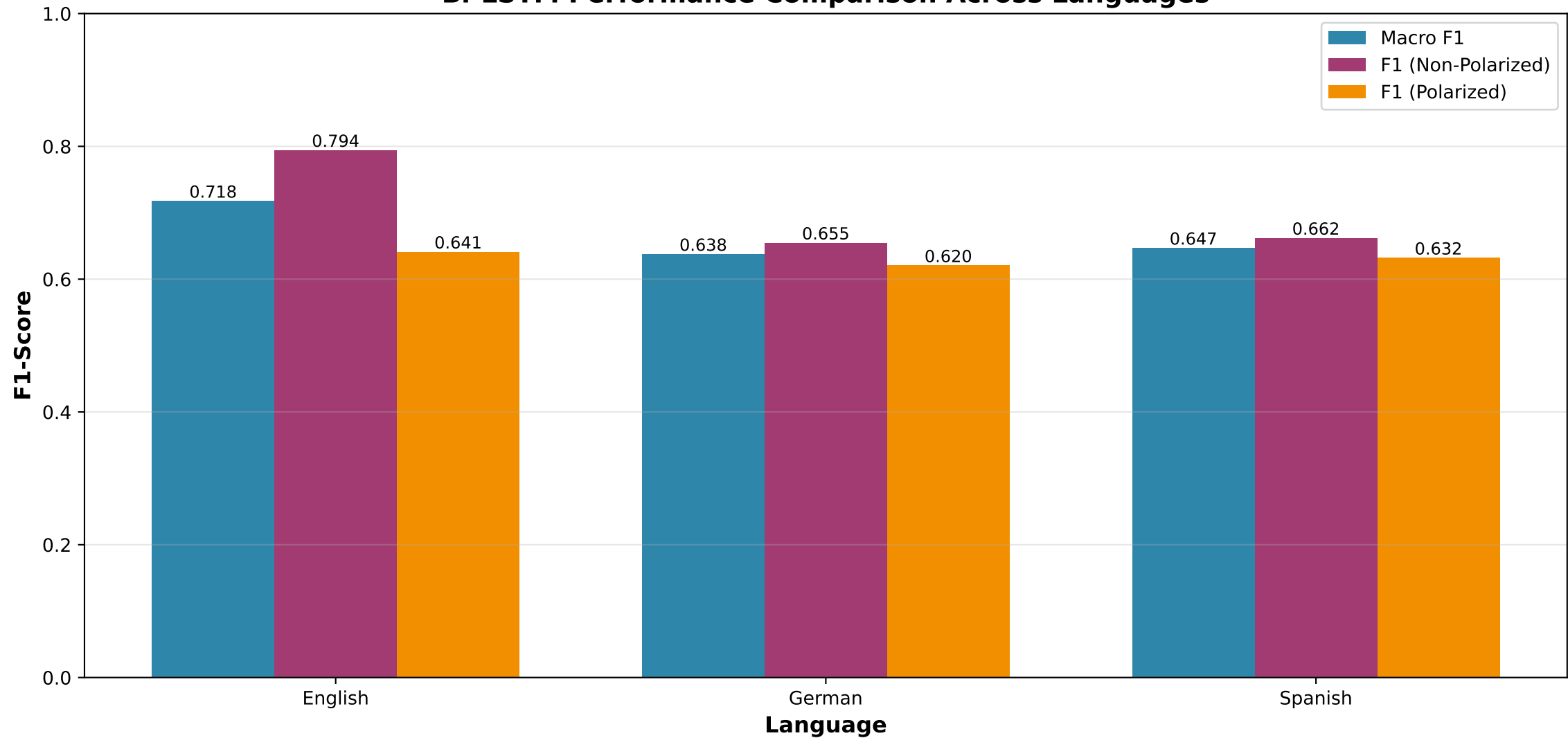
Bi-LSTM Performance Comparison Across Languages
