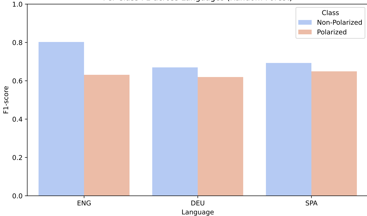
Per-Class F1 across Languages (Random Forest)
