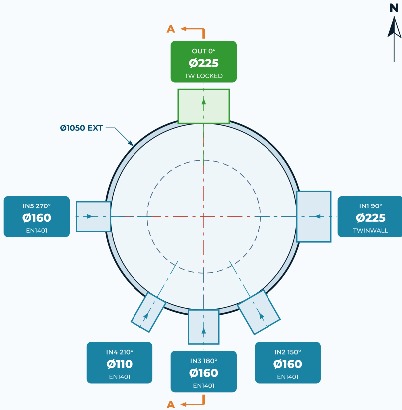
PLAN VIEW (COVER REMOVED) | SCALE 1:20
