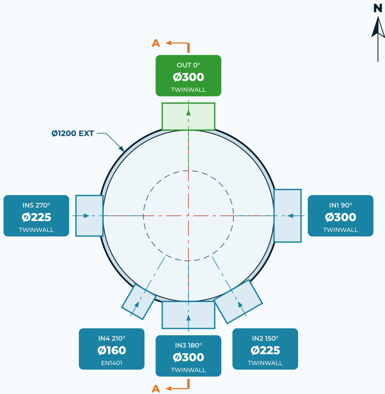
PLAN VIEW (COVER REMOVED) | SCALE 1:25
