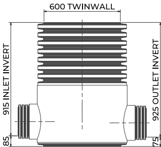
G SERFIC600225-1.0 ELEVATIONS, 1000 MM HIGH NOT TO SCALE
