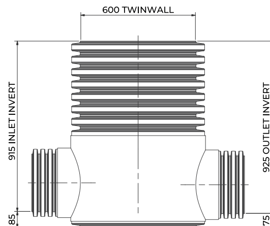
SERFIC600 elevation. Dimensions in mm. NOT TO SCALE
