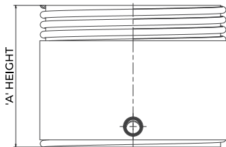
J 750 TO 1200 MM RANGE: A HEIGHT, B INLET INVERT, C OUTLET INVERT NOT TO SCALE
