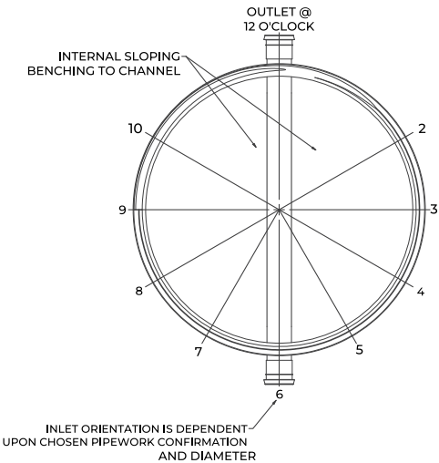
H 1200 MM PLAN AND CLOCK POSITIONS NOT TO SCALE
