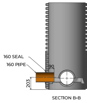
M SIDE INLET SECTIONS, 600 MM CHAMBER
