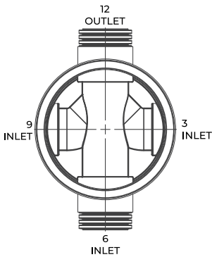
F SERFIC600225-1.0 PLAN NOT TO SCALE
