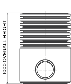
G SERFIC600225-1.0 ELEVATIONS, 1000 MM HIGH NOT TO SCALE
