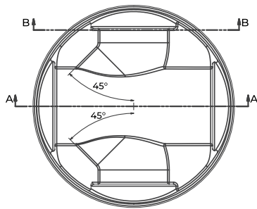
K 3-INLET BASE SEB600-225-225
