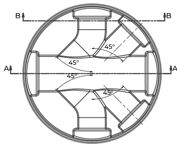
L 5-INLET BASE SEB600-150-150-150
