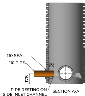
M SIDE INLET SECTIONS, 600 MM CHAMBER
