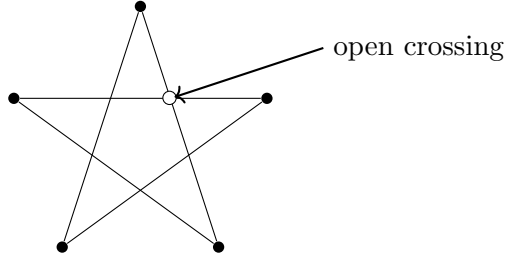
Figure 2: A star-shaped C_5 cycle thrackle with an indicated open crossing.
