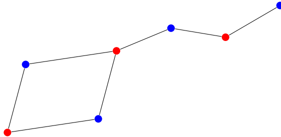
Figure 1: A two-colored bipartite Big Dipper graph consisting of a C_4 cycle with a path attached to one vertex.
