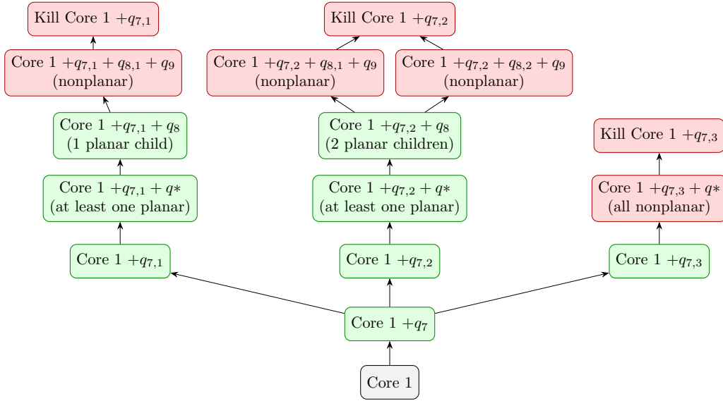
Figure 7: Schematic illustration of the branching search and endpoint pruning. Green nodes indicate states for which at least one planar selected restriction survives. Red nodes indicate states whose continuations are eliminated. Here, q denotes an edge of C_8 , and q^* denotes a distinct later edge tested for lookahead.
