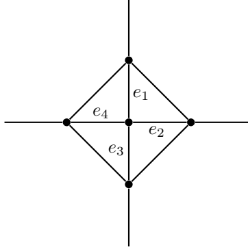
Figure 5: An open crossing vertex surrounded by its diamond configuration lock.
