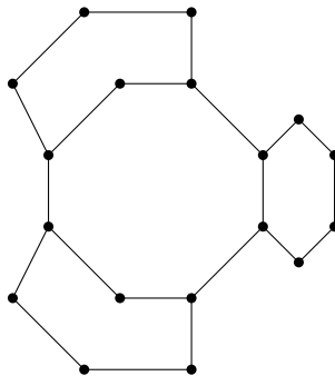
Figure 4: An 8-face with five half-edges, adapted from Xu [Xu21].
