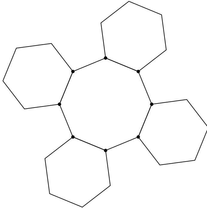
Figure 11: An 8-face with alternating half-edges and non-half-edges, giving the pattern HNHNHNHN .
