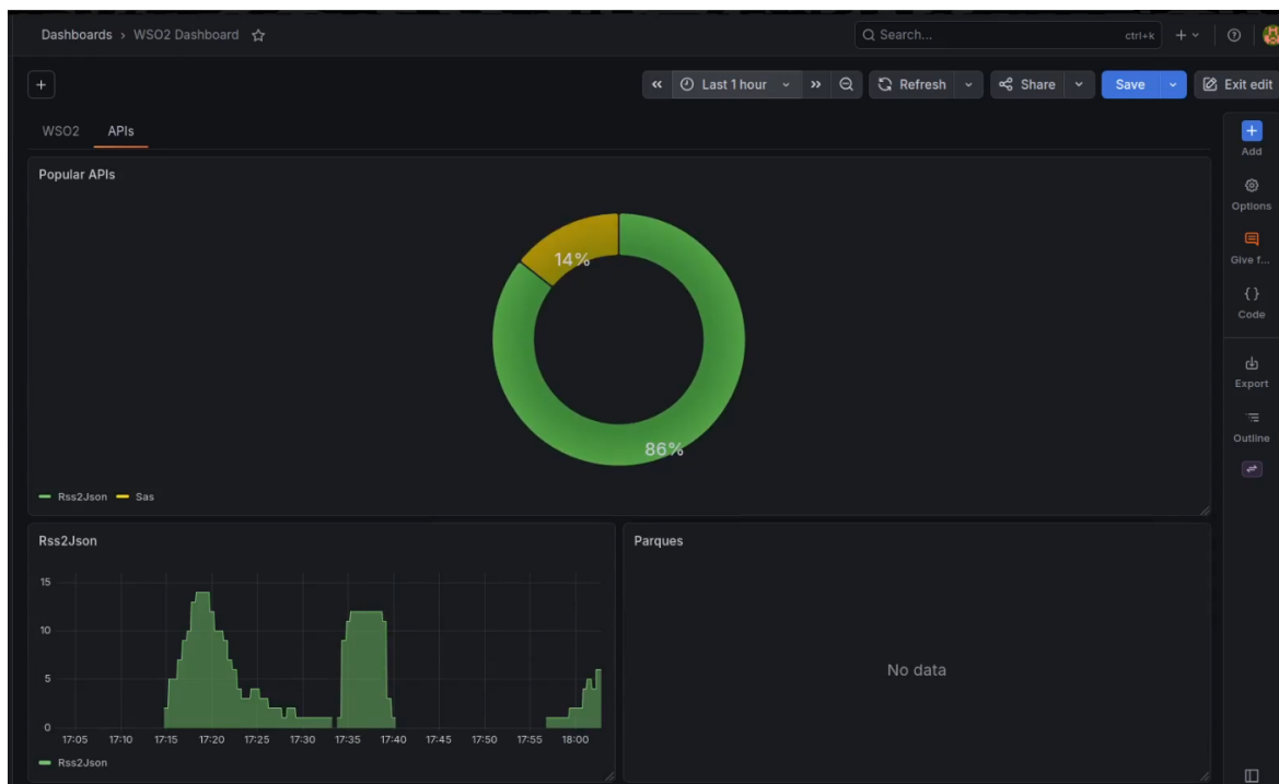
Figure 4.2: Grafana APIs Dashboard — traffic distribution and per-endpoint usage
