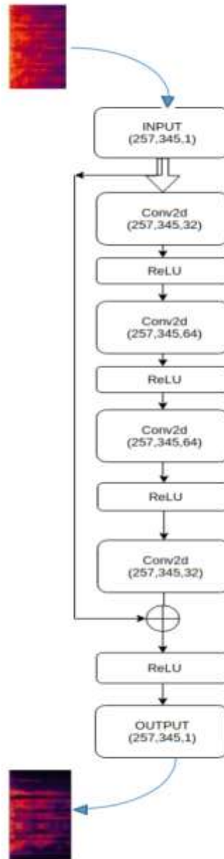
Fig 5.1 System Architecture
