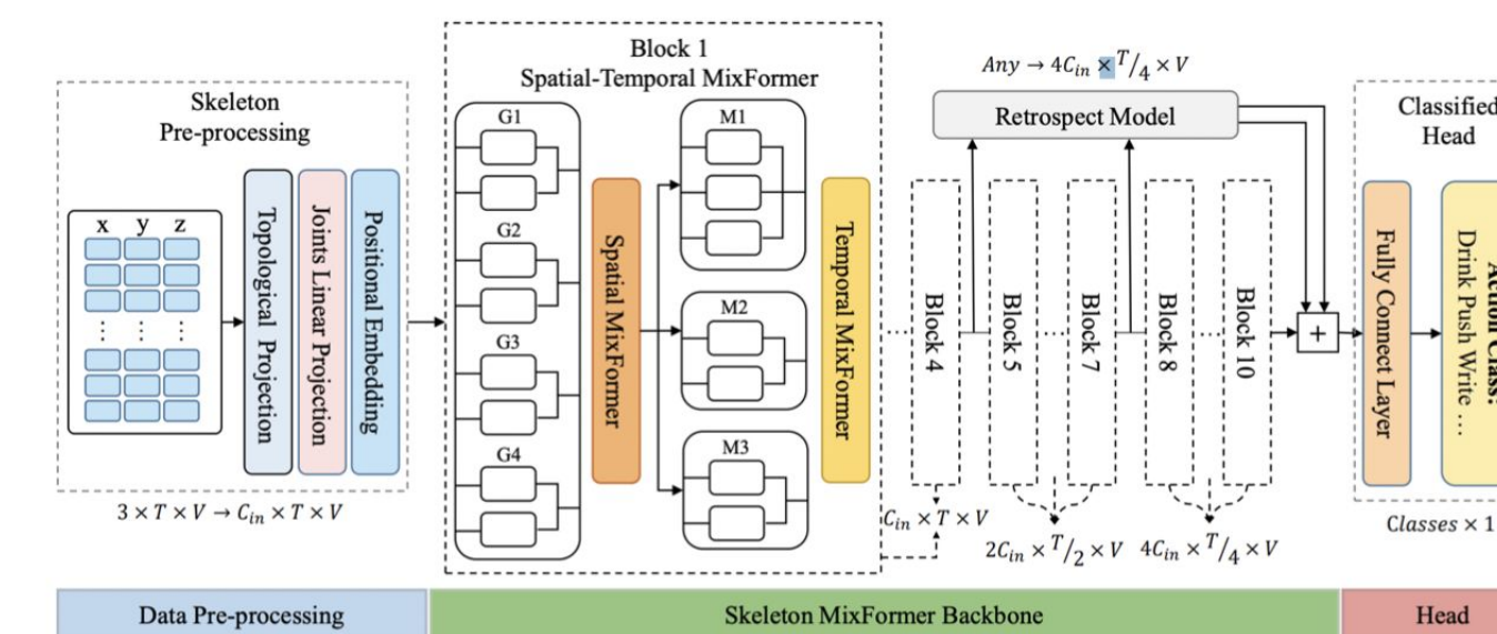
Figure 5: Overall Framework for Skeleton-MixFormer
