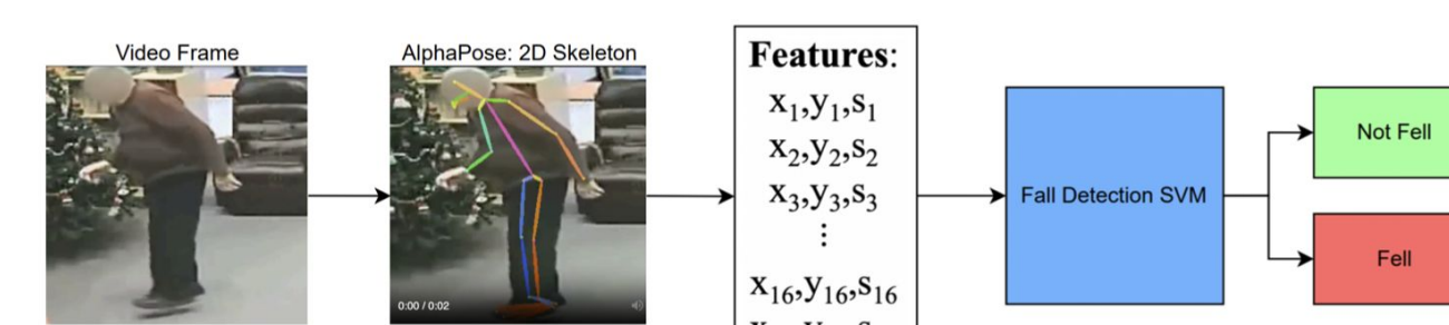
Figure 4: Workflow of the baseline support vector machine (SVM) fall detector. Each video frame is processed by AlphaPose to generate 2D joint coordinates and confidence scores, which form a 51-dimensional feature vector. Recursive feature elimination (RFE) is implemented to identifies the most informative joints for retraining.
