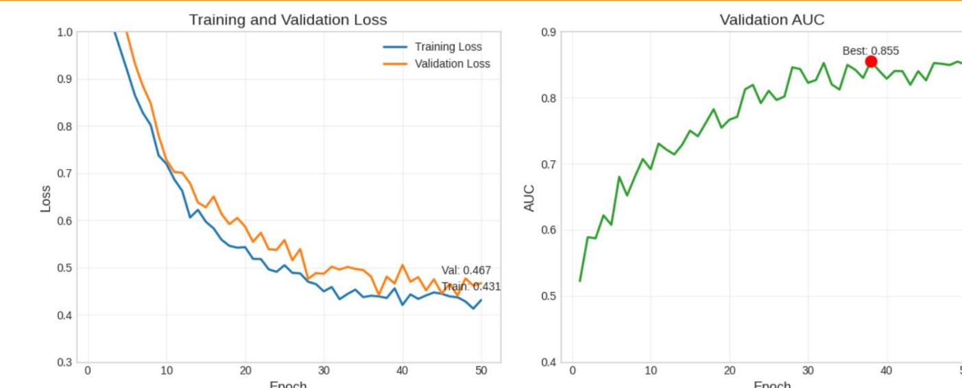
Figure 7: Training and validation loss and AUC curves for TriFallNet Stage 1 over 50 epochs. The best validation AUC attained is 0.855 during epoch 39 and the final validation loss is 0.467. Both curves converge smoothly and have a relatively small gap, indicating effective learning with minimal overfitting.
