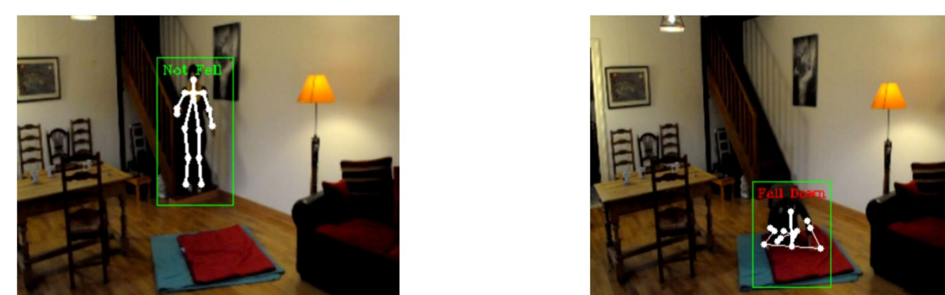
Figure 6: Example visualizations of the baseline SVM outputs on a Le2i video. Left: a non-fall frame correctly classified as "not fell". Right: a fall frame correctly classified as "fell".
