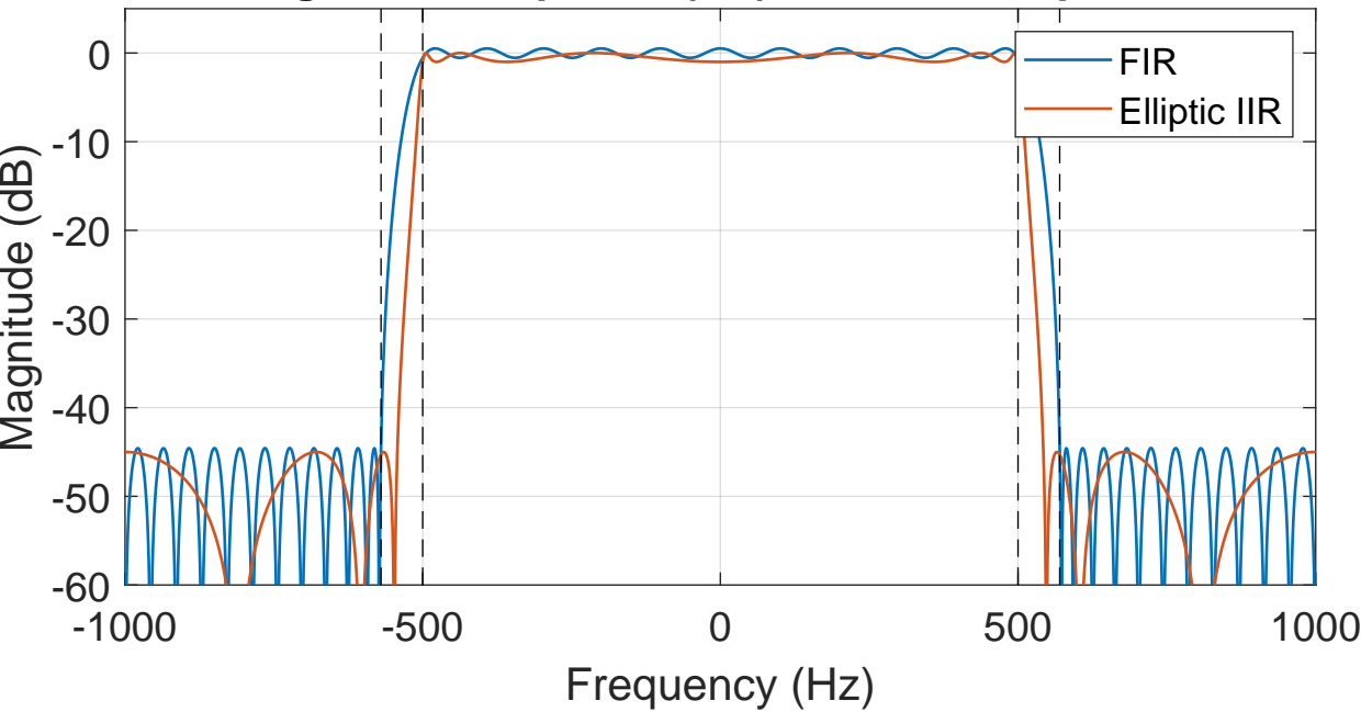
Magnitude response (dB) — FIR vs Elliptic IIR
