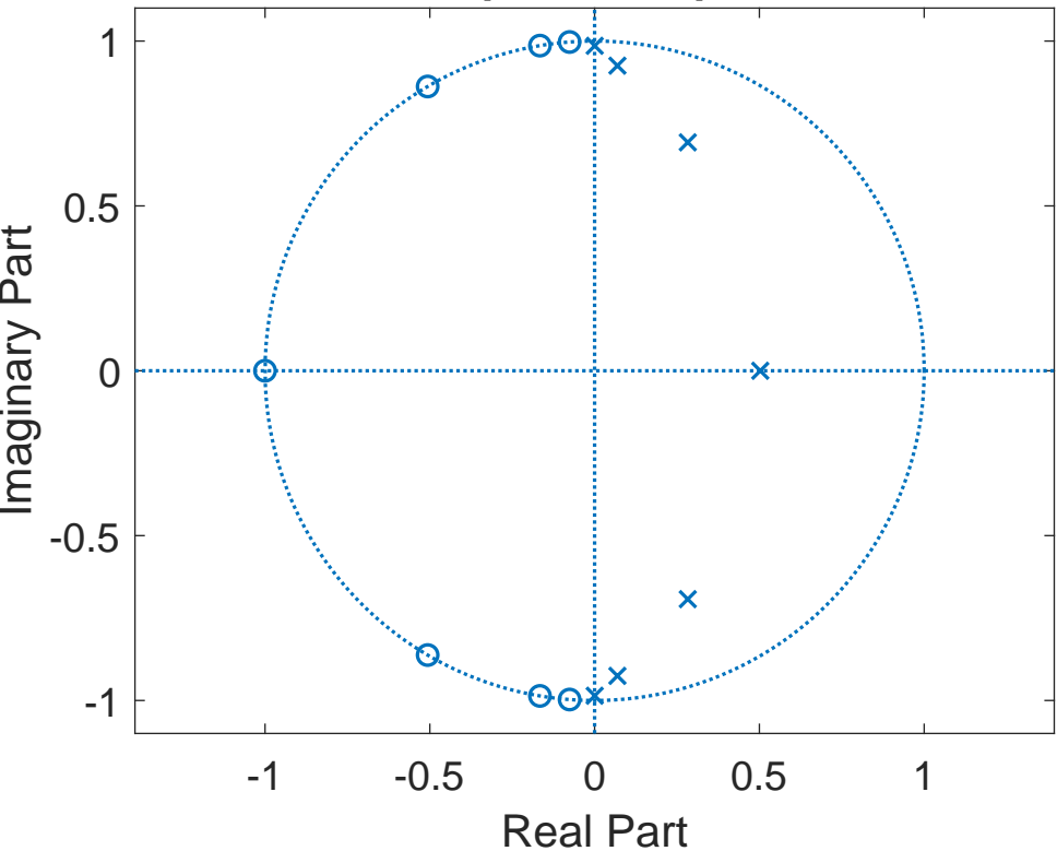
IIIR pole-zero plot
