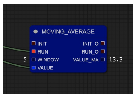
Figure 5.11: Watching an output slot in the Graph View
