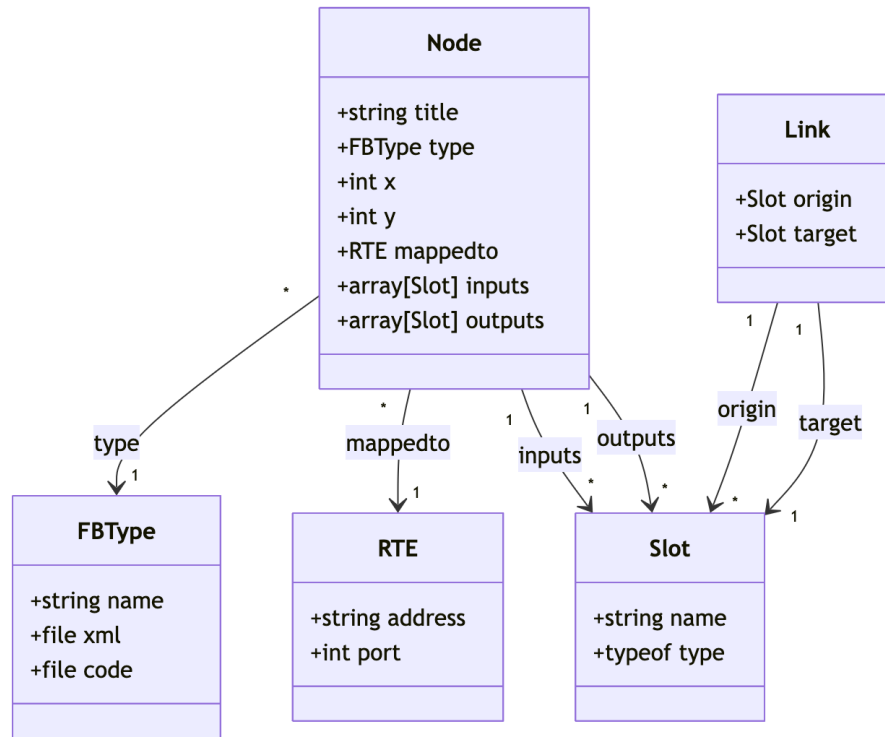
Figure 4.2: Class diagram of the program's data
