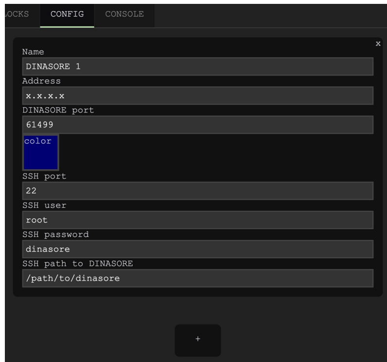
Figure 5.2: Devices Configuration View
