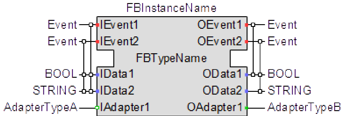
Figure 1.1: IEC 61499 function block interface [8]
