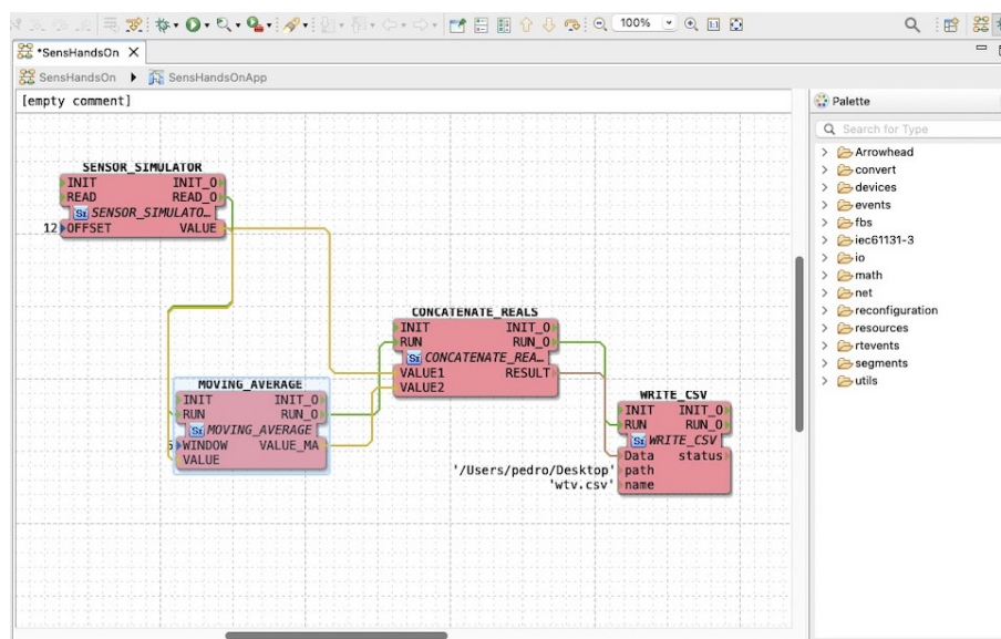
Figure 1.2: 4diac IDE [1]
