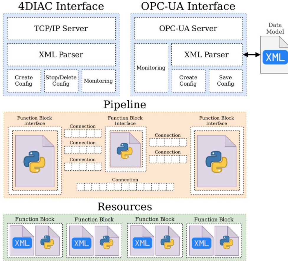
Figure 4.1: DINASORE 's architecture [27].
