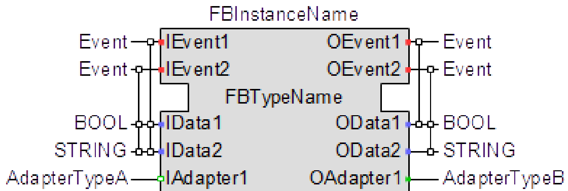
Figure 1.1: IEC 61499 function block interface [11]
