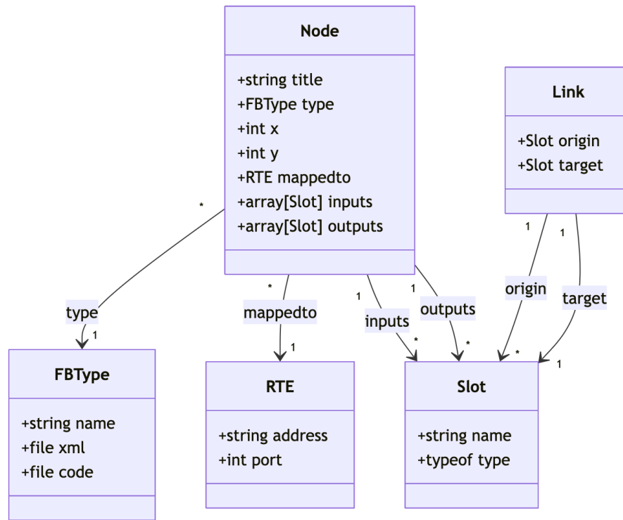
Figure 3.2: Class diagram of the program's data
