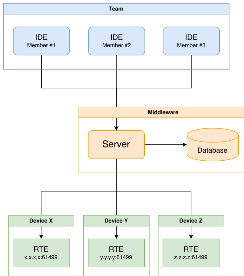
Figure 3.1: Communication through the server
