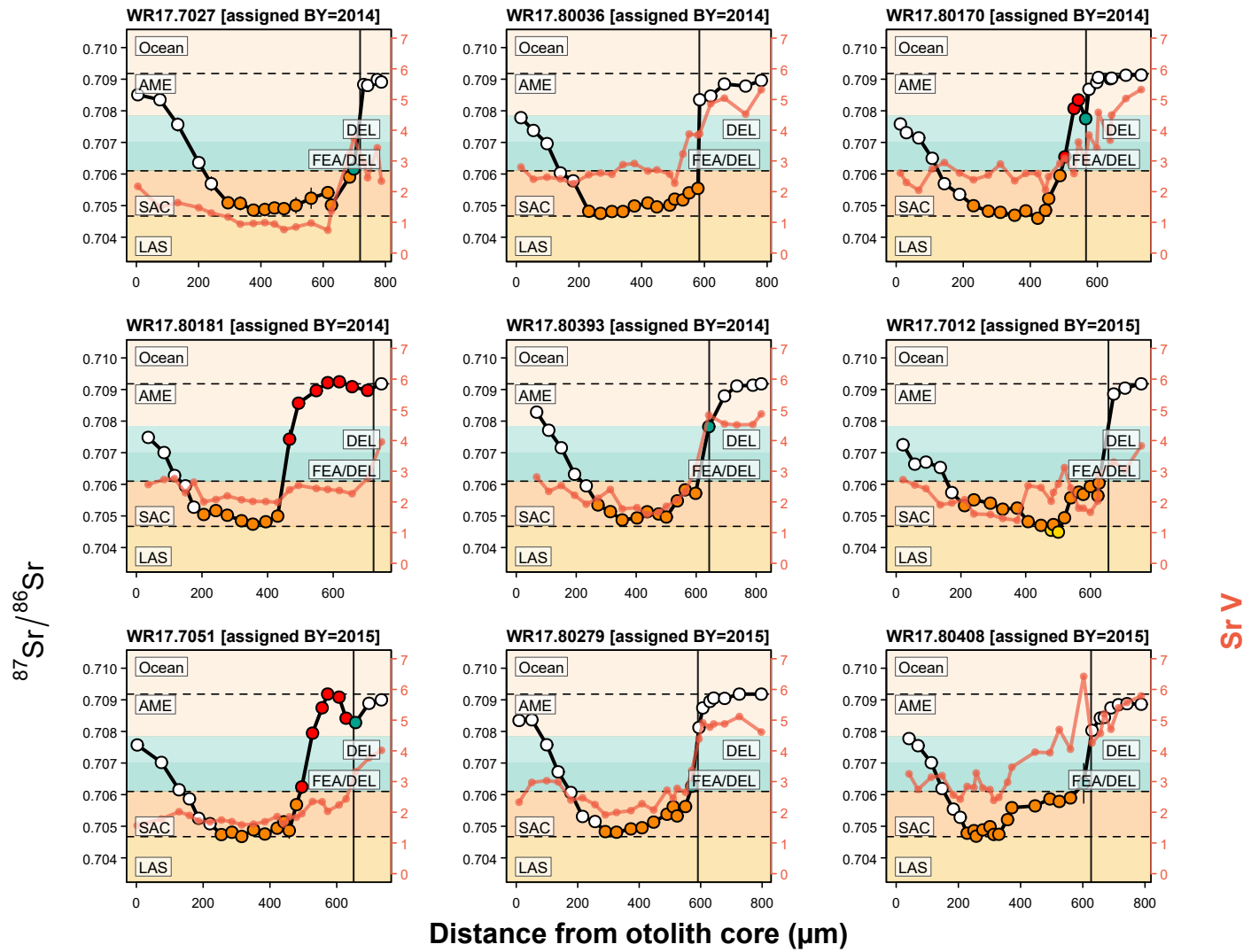
Figure S1. Individual otolith strontium-isotope profiles of juvenile winter-run Chinook salmon. Each panel presents the profile of an individual fish, identified by sample code and assigned brood year. The normalized otolith ^{87}\text{Sr}/^{86}\text{Sr} ratio (black line and points; left y-axis) and Sr signal in volts (light red line and points; right y-axis) are plotted against distance from the otolith core ( \mu\text{m} ). Vertical error bars around ^{87}\text{Sr}/^{86}\text{Sr} measurements represent \pm 2 SE (standard error). Point colors indicate habitat assignments: Lassen Tributaries (LAS), Sacramento River (SAC), Feather River or Delta (FEA/DEL), American River (AME), Delta (DEL), and unassigned. Shaded horizontal bands represent the reference ^{87}\text{Sr}/^{86}\text{Sr} ranges associated with LAS, SAC, FEA/DEL, AME, and DEL habitats. Horizontal dashed lines denote boundaries between selected habitat ranges and also with the ocean reference threshold. The solid vertical black line indicates the estimated distance from the otolith core at freshwater exit.
