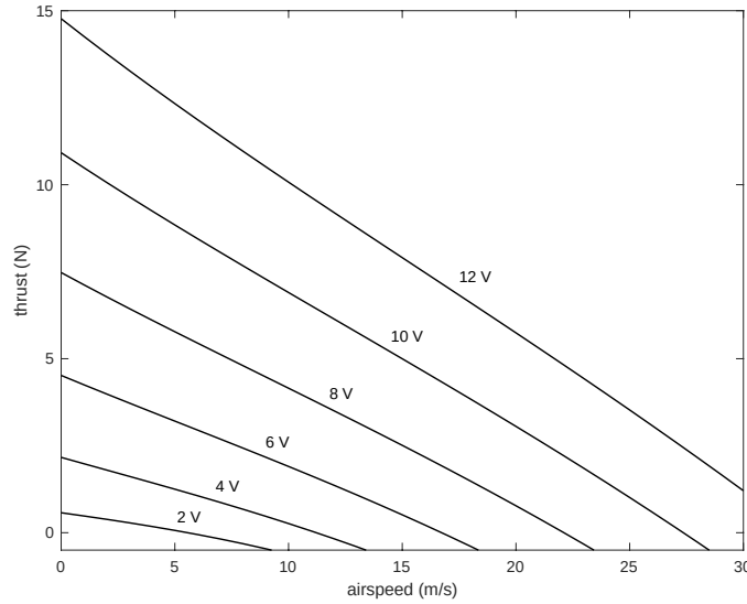
Figure 4.11: Propeller thrust versus airspeed for various motor voltage settings.
