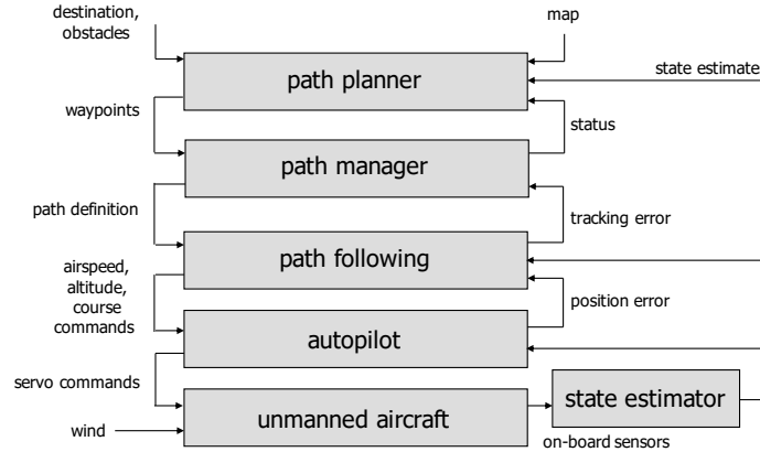
Figure 1.1: The system architecture that will be assumed throughout the book. The path planner produces straight-line or Dubins paths through an obstacle field. The path manager switches between orbit following and straight-line path following to maneuver along the waypoint paths. The path-following block produces commands to the low-level autopilot, which controls the airframe. Each of the blocks relies on estimates of the states produced by filtering the onboard sensors.
