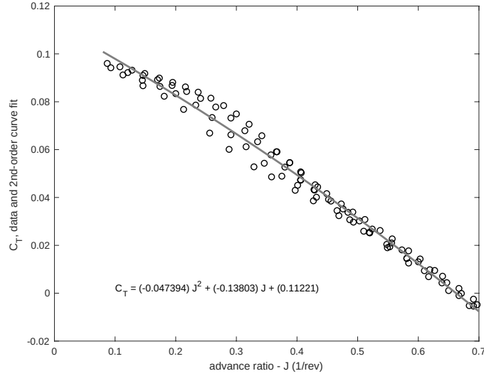
Figure 4.9: Thrust coefficient versus advance ratio for APC Thin Electric 10x5 propeller [22].
