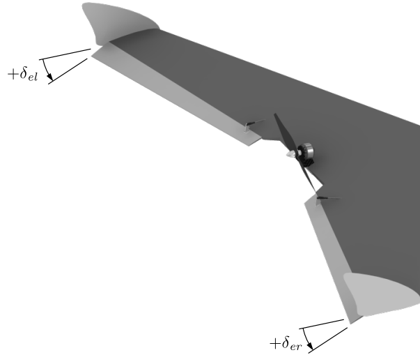
Figure 4.5: Elevons are used to control a flying-wing aircraft. The elevons replace the aileron and the elevator. Driving the elevons together has the same effect as an elevator, and driving them differentially has the same effect as ailerons.
