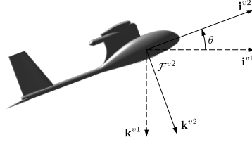
Figure 2.5: The vehicle-2 frame. The \mathbf{i}^{v2} -axis points out the nose of the aircraft, the \mathbf{j}^{v2} -axis points out the right wing, and the \mathbf{k}^{v2} -axis points out the belly.
