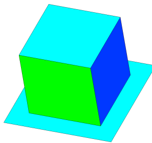
Figure D.7: Rendering of the spacecraft using vertices and faces.
