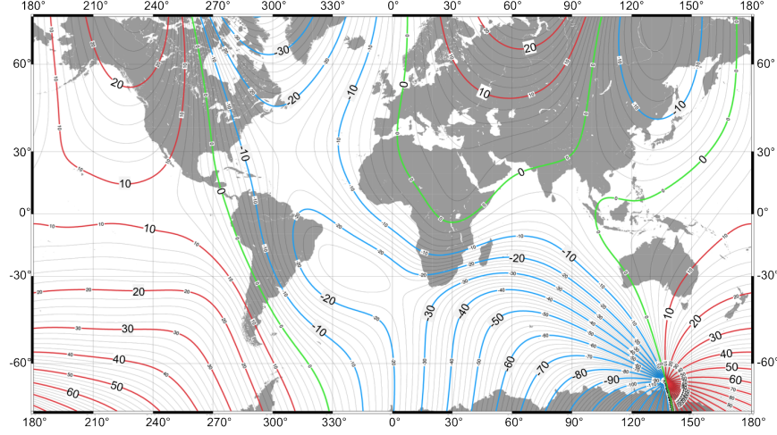
Figure 7.7: Lines of constant declination angles \delta of the earth's magnetic field, according to the US/UK World Magnetic Model. Adapted from [47].
