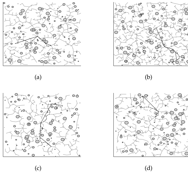
Figure 12.8: The results of algorithm 13 for four randomly generated obstacle fields and randomly generated start and end nodes are indicated by dashed lines. The smoothed paths generated by algorithm 14 are indicated by the solid lines.
