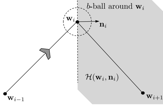
Figure 11.1: When transitioning from one straight-line segment to another, a criterium is needed to indicate when the MAV has completed the first straight-line segment. A possible option is to switch when the MAV enters a b -ball around the transition waypoint. A better option is to switch when the MAV enters the half-plane \mathcal{H}(\mathbf{w}_i, \mathbf{n}_i) .
