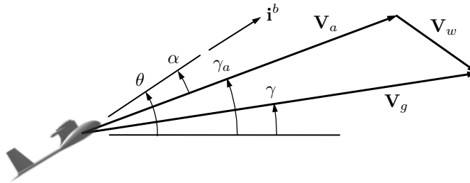
Figure 2.11: The wind triangle projected onto the vertical plane.
