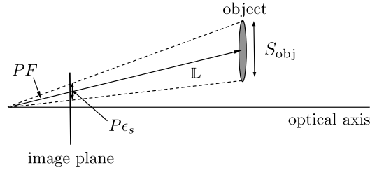
Figure 13.5: The size and growth of the target in the image frame can be used to estimate the time to collision.
