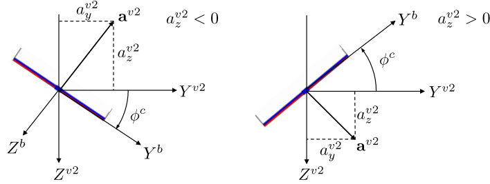
Figure 13.7: Polar converting logic that transforms an acceleration command \mathbf{a}^{v2} to a commanded roll angle \phi^c and a commanded normal acceleration V_g \dot{\gamma}^c .
