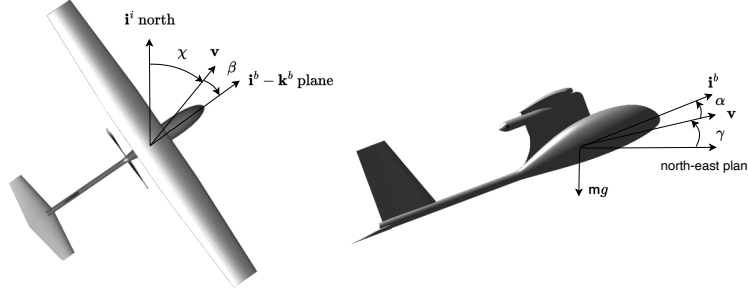
Figure 9.3: The course angle \chi is the angle between the inertial north axis and the projection of the velocity vector \mathbf{v}_g onto the north-east plane. The side-slip angle \beta is the angle between the velocity vector \mathbf{v}_g and the body \mathbf{i}^b - \mathbf{k}^b plane. The flight path angle \gamma is the angle between the inertial north-east plane and the velocity vector \mathbf{v}_g . The angle-of-attack \alpha is the angle between the body \mathbf{i}^b axis and the projection of the velocity vector \mathbf{v}_g onto the body \mathbf{i}^b - \mathbf{k}^b plane.
