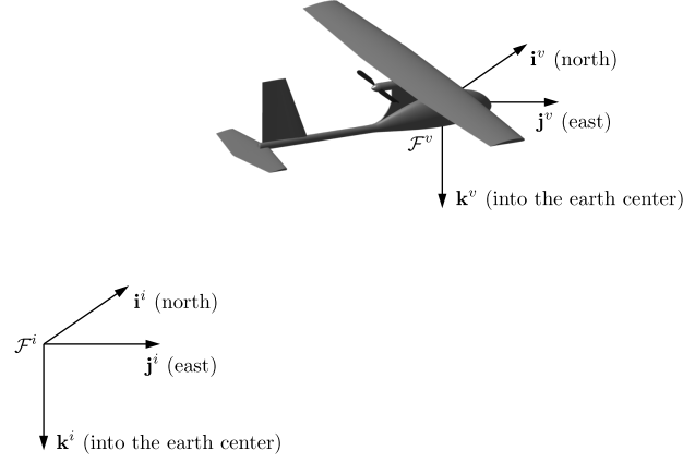
Figure 2.3: The inertial coordinate frame and the vehicle coordinate frame. The \mathbf{i}^i and \mathbf{i}^v -axes points north , the \mathbf{j}^i and \mathbf{j}^v -axes points east , and the \mathbf{k}^i and \mathbf{k}^v -axis points into the earth. The inertial frame is located at a fixed location usually on the ground. The origin of the vehicle frame is at the center of mass of the MAV.
