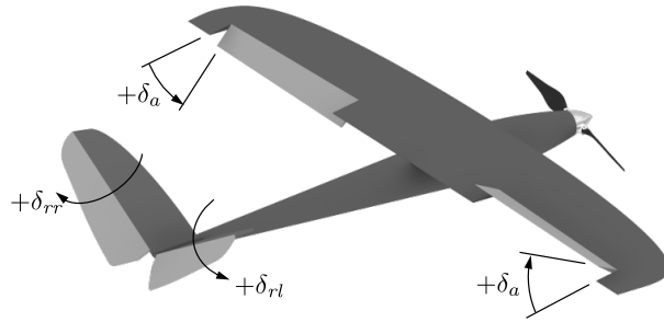
Figure 4.4: Ruddervators are used to control a v-tail aircraft. The ruddervators replace the rudder and the elevator. Driving the ruddervators together has the same effect as an elevator, and driving them differentially has the same effect as a rudder.
