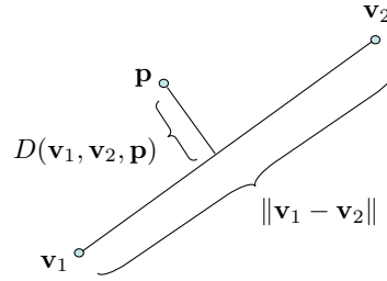
Figure 12.3: The cost penalty assigned to each edge of the Voronoi graph is proportional to the path length \|v_1 - v_2\| and the reciprocal of the minimum distance from the path to a point in Q .
