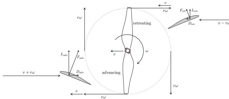
Figure 14.5: Induced drag on a propeller.
