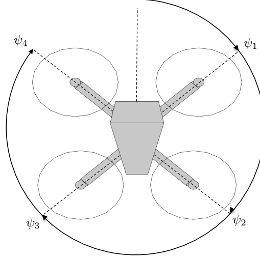
Figure 14.8: The top view of a quadrotor where the motor arms each of length \ell and are equally spaced angularly.
