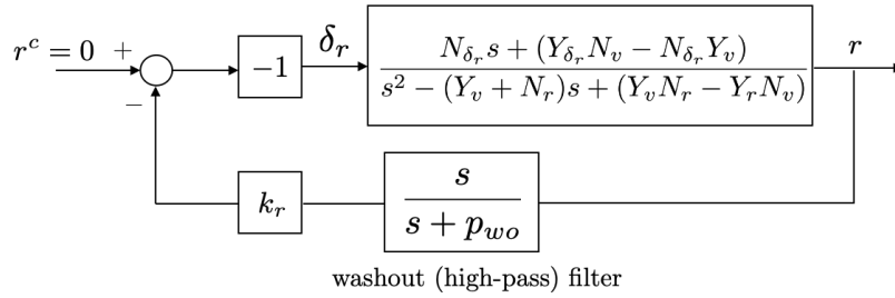
Figure 6.9: Yaw damper with washout filter.
