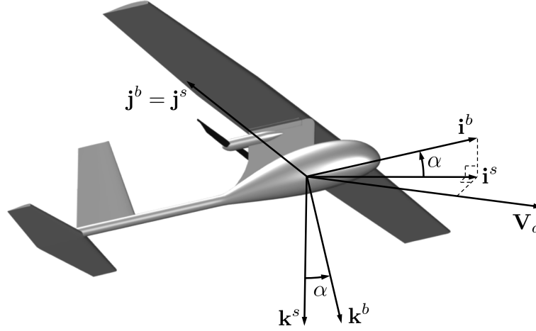
Figure 2.7: The stability frame. The \mathbf{i}^s -axis points along the projection of the airspeed vector onto the \mathbf{i}^b - \mathbf{k}^b plane of the body frame, the \mathbf{j}^s -axis is identical to the \mathbf{j}^b -axis of the body frame, and the \mathbf{k}^s -axis is constructed to make a right-handed coordinate system. The angle-of-attack is defined as a right-handed rotation about the body \mathbf{j}^s -axis.
