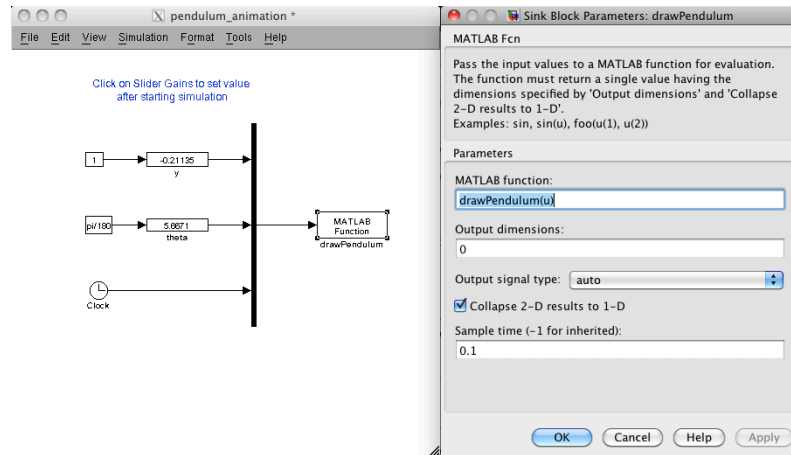
Figure D.3: Simulink file for debugging the pendulum simulation. There are three inputs to the Matlab m-file drawPendulum : the position y , the angle \theta , and the time t . Slider gains for y and \theta are used to verify the animation.
