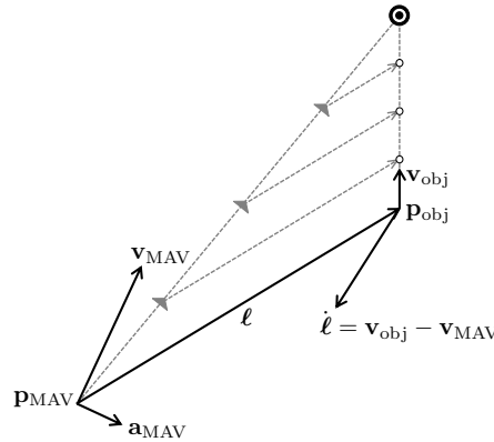
Figure 13.6: The geometry associated with precision landing.
