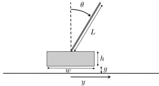
Figure D.2: Drawing for inverted pendulum. The first step in developing an animation is to draw a figure of the object to be animated and identify all of the physical parameters.
