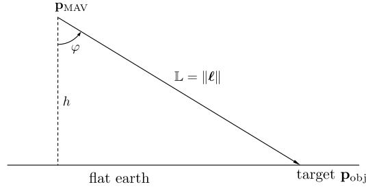
Figure 13.3: Range estimation using the flat-earth assumption.
