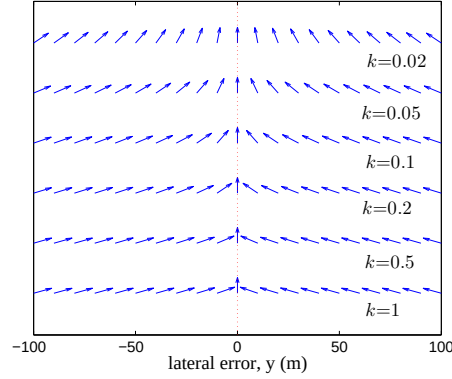
Figure 10.4: Vector fields for various values of k_{\text{path}} . Large values of k_{\text{path}} yield abrupt transitions from \chi^\infty to zero, while small values of k_{\text{path}} give smooth transitions.
