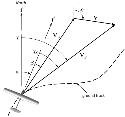
Figure 2.10: Heading is the direction that the MAV is pointed. Course is the direction of travel relative to the earth's surface. The crab angle is the difference between course and heading. In the absence of wind, the crab angle is zero.
