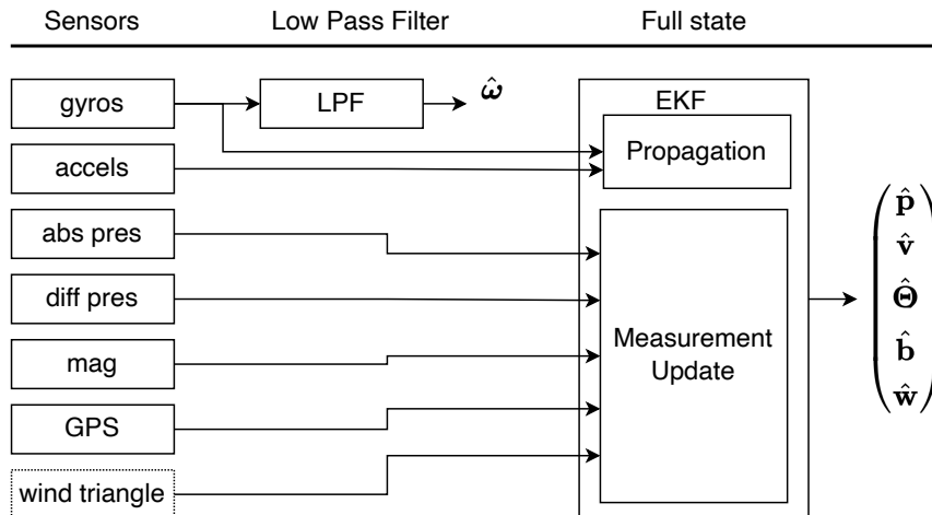
Figure 8.10: Block diagram for the full state extended Kalman filter.
