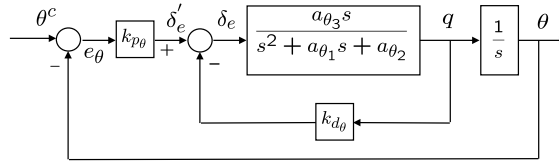
Figure 6.12: Pitch attitude hold feedback loops.
