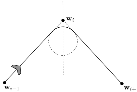
Figure 11.3: The transition from straight-line path \overline{\mathbf{w}_{i-1}\mathbf{w}_i} to \overline{\mathbf{w}_i\mathbf{w}_{i+1}} can be smoothed by inserting a fillet.
