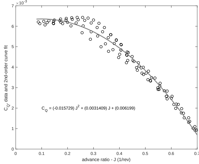
Figure 4.10: Torque coefficient versus advance ratio for APC Thin Electric 10x5 propeller [22].
