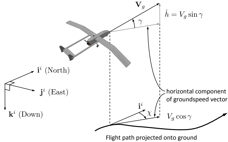
Figure 2.9: The flight path angle \gamma and the course angle \chi .
