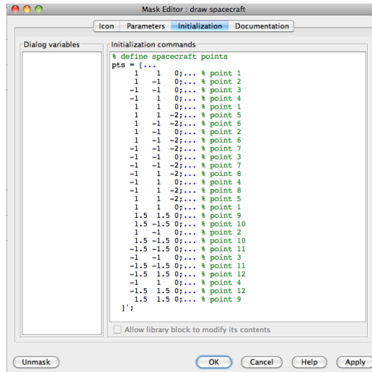
Figure D.6: The mask function in Simulink allows the spacecraft points to be initialized at the beginning of the simulation.
