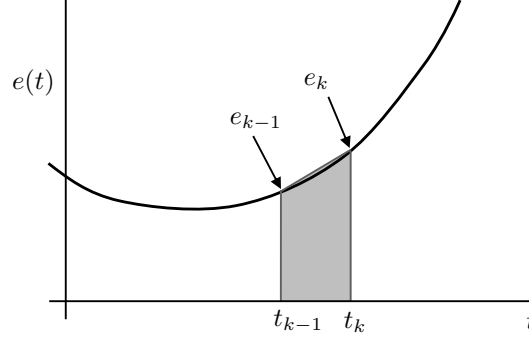
Figure C.1: Discrete approximation of area under the curve using the trapezoidal rule.
