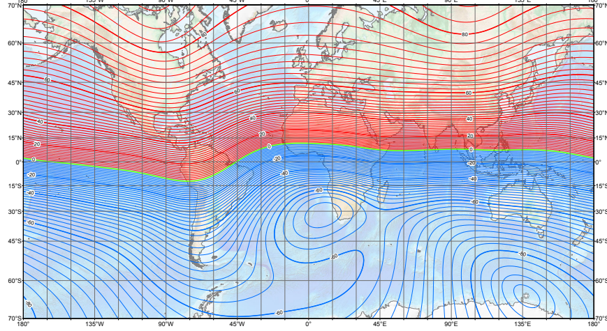
Figure 7.8: Lines of constant inclination angles \iota of the earth's magnetic field, according to the US/UK World Magnetic Model. Adapted from [47].
