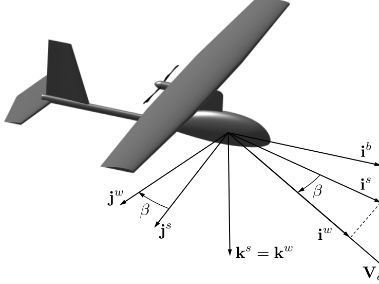
Figure 2.8: The wind frame. The \mathbf{i}^w -axis points along the airspeed vector.
