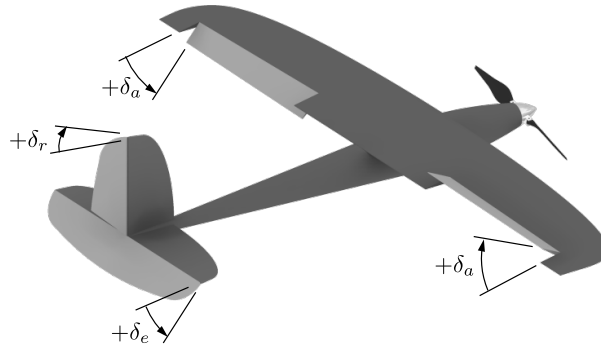
Figure 4.3: Control surfaces for a standard aircraft configuration. The ailerons are used to control the roll angle \phi . The elevators are used to control the pitch angle \theta . The rudder directly effects the yaw angle \psi .
