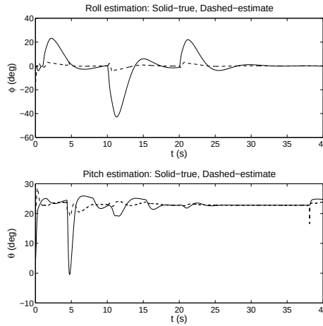
Figure 8.4: Estimation error on the roll and pitch angles obtained by low-pass filtering the accelerometers and inverting the model. Since this scheme assumes unaccelerated flight during maneuvers where acceleration exists, the estimation error can be unacceptably large.
