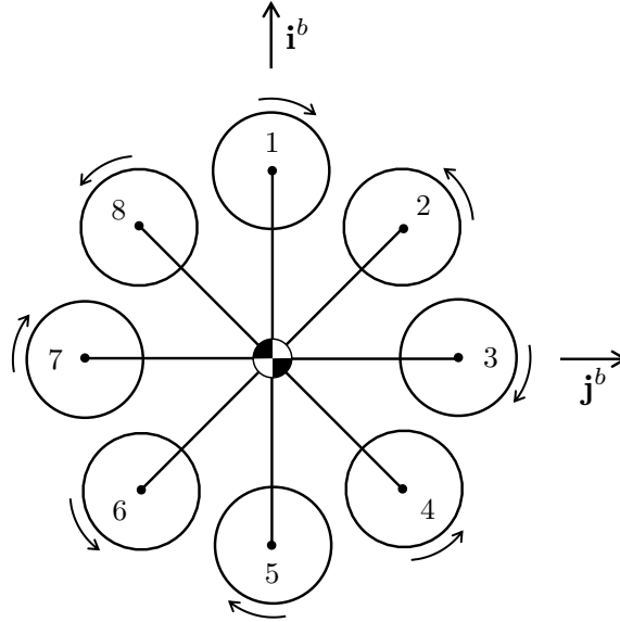
Figure 14.6: Octocopter example of a multirotor configuration.
