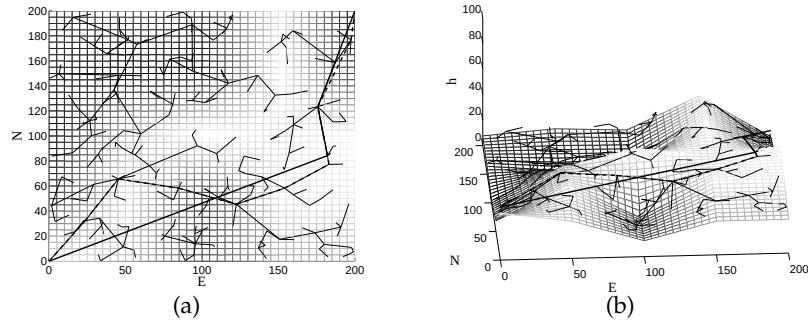
Figure 12.9: (a) Overhead view of the results of the 3-D RRT waypoint path planning algorithm. (b) Side view of the results of the 3-D RRT waypoint path planning algorithm. The thin lines are the RRT graph, the thick dotted line is the RRT path returned by algorithm 13, and the thick solid line is the smoothed path. The RRT graph is generated at a fixed height above the terrain.
