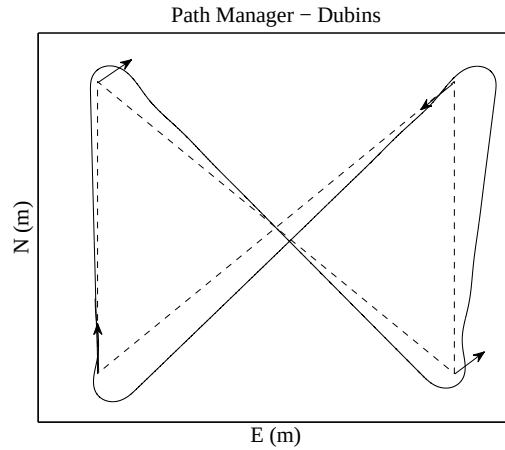
Figure 11.14: An example of the types of flight paths produced by algorithm 11.
