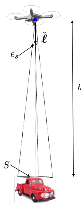
Figure 14.10: Vision-based target tracking from a quadrotor, where \check{\ell} is the measured normalized line-of-sight vector and \epsilon_s is the measured pixel area, and S is the size(area) of the target being tracked..
