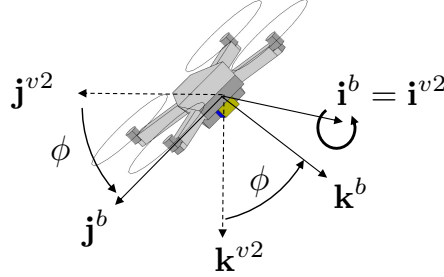
Figure 14.3: The body frame for a multirotor.
