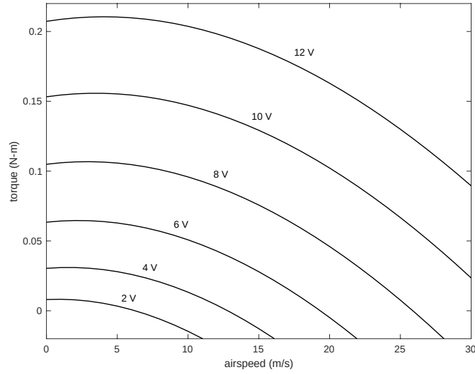
Figure 4.12: Motor torque versus airspeed for various motor voltage settings.
