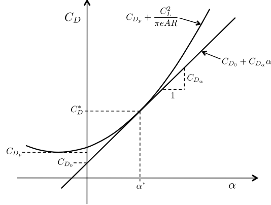
Figure 4.8: The drag coefficient as a function of angle-of-attack . Linear and quadratic models are represented.
