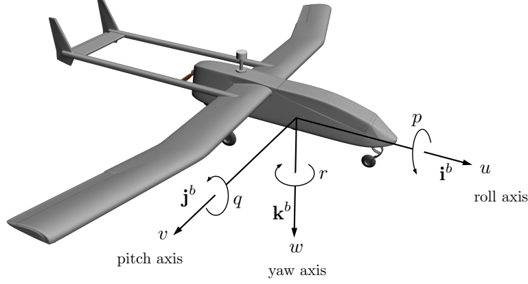
Figure 3.1: Definition of axes of motion.
