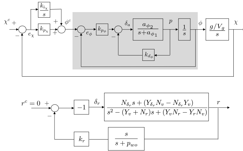
Figure 6.5: Autopilot for lateral control using successive loop closure.
