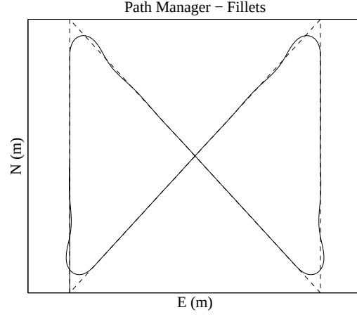
Figure 11.6: An example of the types of flight paths produced by algorithm 9.
