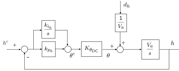
Figure 6.13: The altitude-hold loop using the commanded pitch angle.
