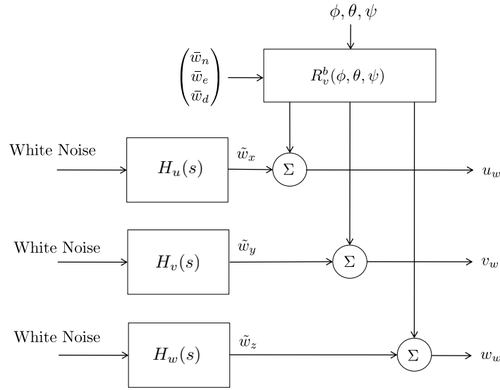
Figure 4.13: The wind is modeled as a constant wind field plus turbulence. The turbulence is generated by filtering white noise with a Dryden model.
