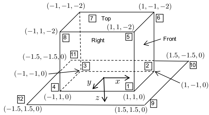
Figure D.1: Simple spacecraft model defining vertices and faces.
