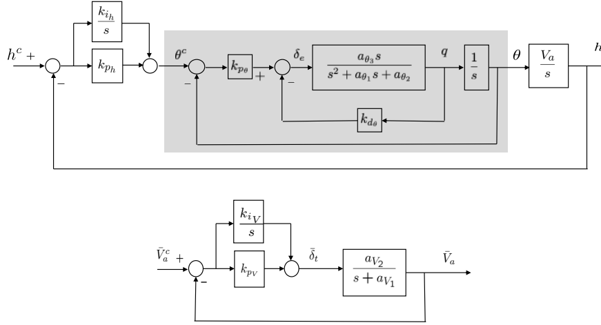
Figure 6.11: Autopilot for longitudinal control using successive loop closure.
