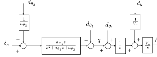
Figure 5.6: Block diagram for longitudinal dynamics.
