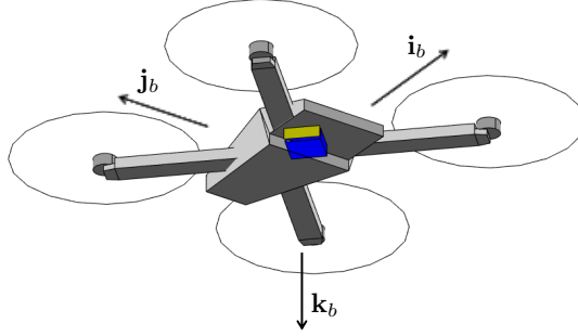
Figure 14.4: Quadrotor with body-frame axes that coincide at the center of mass.
