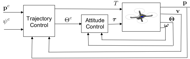
Figure 14.9: Architecture for the control of a multirotor UAV.
