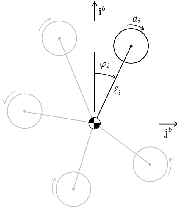
Figure 14.7: Definition of rotor configuration variables.
