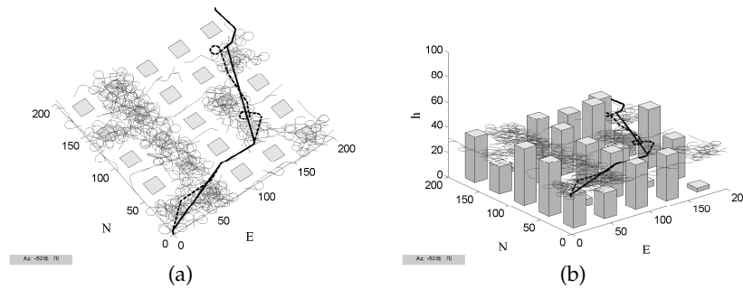
Figure 12.12: (a) Overhead view of the results of the 3-D RRT waypoint path planning algorithm. (b) Side view of the results of the 3-D RRT waypoint path planning algorithm. The thin lines are the RRT graph, the thick dashed line is the RRT path returned by algorithm 13, and the thick solid line is the smoothed path. The RRT graph is generated at a fixed height above the terrain.
