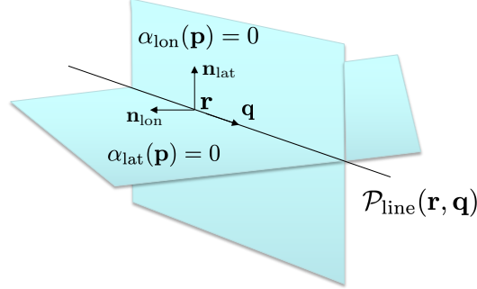
Figure 10.8: This figure shows how the straight-line path \mathcal{P}_{\text{line}}(\mathbf{r}, \mathbf{q}) is defined by the intersection of the two surfaces given by \alpha_{\text{lon}}(\mathbf{p}) = 0 and \alpha_{\text{lat}}(\mathbf{p}) = 0 .
