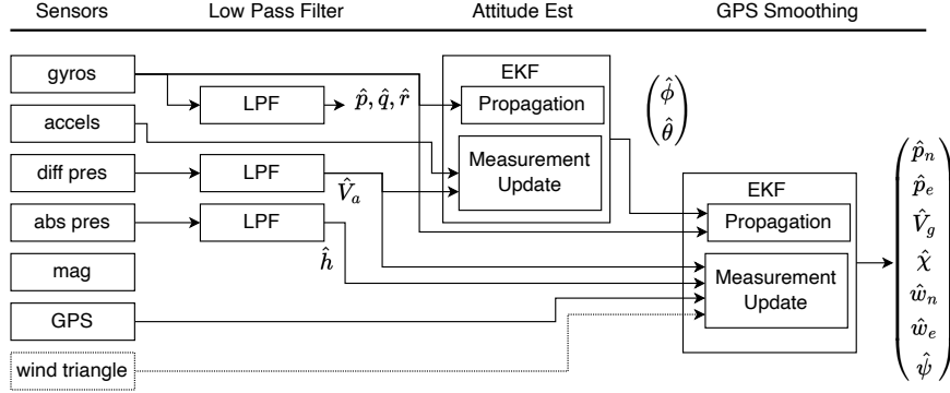
Figure 8.7: Block diagram for the two-stage extended Kalman filter. In the first stage, an EKF is used to estimate the roll and pitch angles from rate gyros and accelerometers. In the second stage, GPS is used to estimate position, groundspeed, course, wind, and heading.
