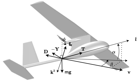
Figure 9.2: Free-body diagram indicating external forces impacting the evolution of the magnitude of velocity. L is lift, D is drag, T is thrust, and g is the gravity vector.
