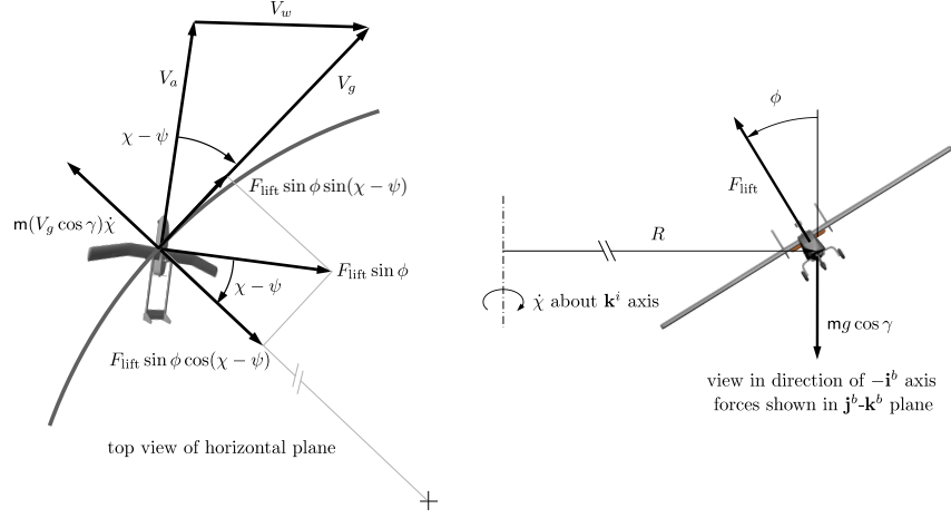
Figure 5.1: Free-body diagram indicating forces on a MAV in a climbing coordinated turn. The MAV is flying at a flight path angle of \gamma with the nose of the MAV directed out of the page. The forces shown are in the \mathbf{j}^b\text{-}\mathbf{k}^b plane.
