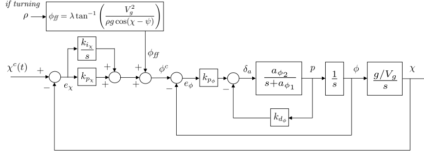
Figure 10.7: Lateral-directional control block diagram with roll feedforward command for orbit tracking.
