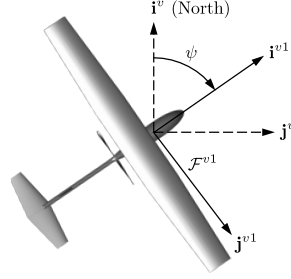
Figure 2.4: The vehicle-1 frame. The \mathbf{i}^{v1} -axis points out the nose of the aircraft, the \mathbf{j}^{v1} -axis points out the right wing, and the \mathbf{k}^{v1} -axis points into the earth.
