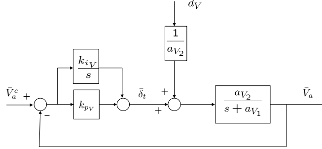
Figure 6.14: Airspeed hold using throttle.
