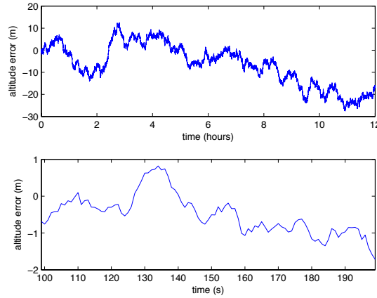
Figure 7.10: Example GPS altitude position error from Gauss-Markov model.
