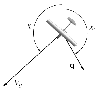
Figure 10.5: The calculation of \chi_q needs to account for the current course angle of the MAV. In this scenario, the MAV should turn left to align with the waypoint path, but if \chi_q is computed with \text{atan2} , the angle will be a positive number slightly smaller than +\pi , which will cause the MAV to turn right to align with the waypoint path.
