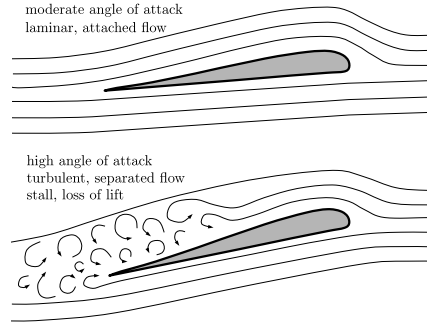
Figure 4.6: The upper drawing depicts a wing under normal flow conditions. The flow is laminar and follows the surface of the wing. The lower drawing shows a wing under stall conditions due to a high angle-of-attack . In this case, the flow separates from the top surface of the wing, leading to turbulent flow and a significant drop in the lift force produced by the wing.
