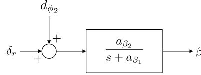
Figure 5.4: Block diagram for the rudder-sideslip dynamics.
