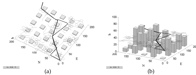
Figure 12.11: (a) Overhead view of the results of the RRT Dubins path planning algorithm. (b) Side view of the results of the RRT Dubins path planning algorithm. The thin lines are the RRT graph, the thick dashed line is the RRT path returned by algorithm 13, and the thick solid line is the smoothed path. The RRT graph is generated at a fixed height above the terrain.
