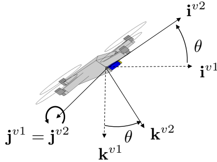
Figure 14.2: The vehicle-2 frame for a multirotor.
