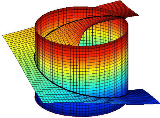
Figure 10.9: A helical path for parameters \mathbf{c} = (0, 0, 0)^\top , \rho = 30 m, \lambda = +1 , \chi_h = 0 , and \gamma_h = \frac{15\pi}{180} rad.
