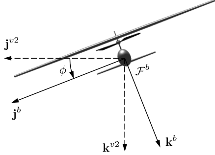
Figure 2.6: The body frame. The \mathbf{i}^b -axis points out the nose of the airframe, the \mathbf{j}^b -axis points out the right wing, and the \mathbf{k}^b -axis points out the belly.
