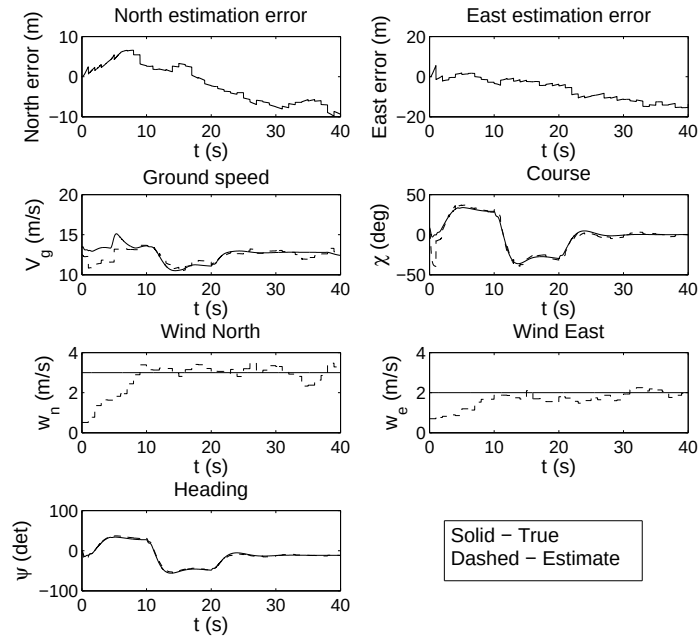
Figure 8.9: Estimation error for position, ground speed, course, wind, and heading using continuous-discrete extended Kalman filter.
