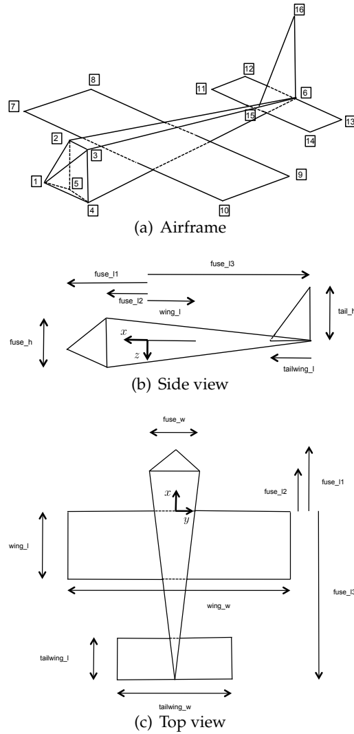
Figure 2.13: Specifications for animation of aircraft for the design project.
