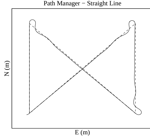
Figure 11.2: Path generated using the path-following approach given in algorithm 8. The MAV follows the straight-line path until reaching the waypoint, and then maneuvers onto the next straight-line section.
