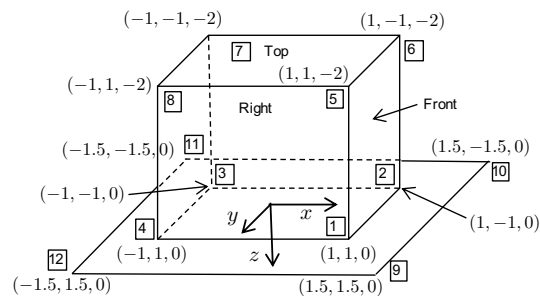
Figure D.4: Drawing used to create spacecraft animation. Standard aerodynamics body axes are used, where the x -axis points out the front of the spacecraft, the y -axis points to the right, and the z -axis point out the bottom of the body.
