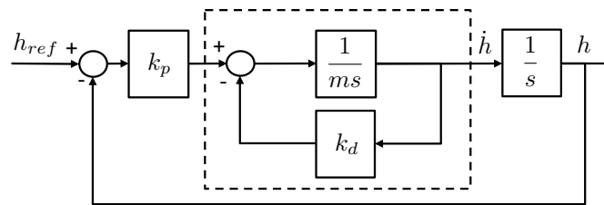
Fig. 2: Height control scheme 1
