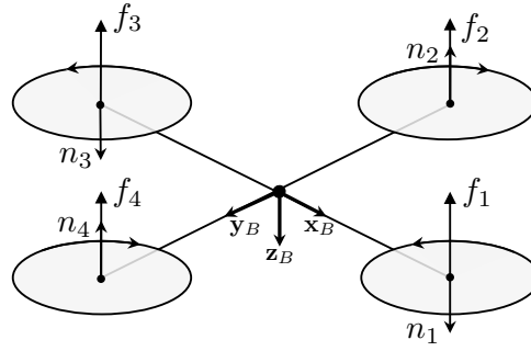
Fig. 1: Simplified model of the Parrot AR.Drone
