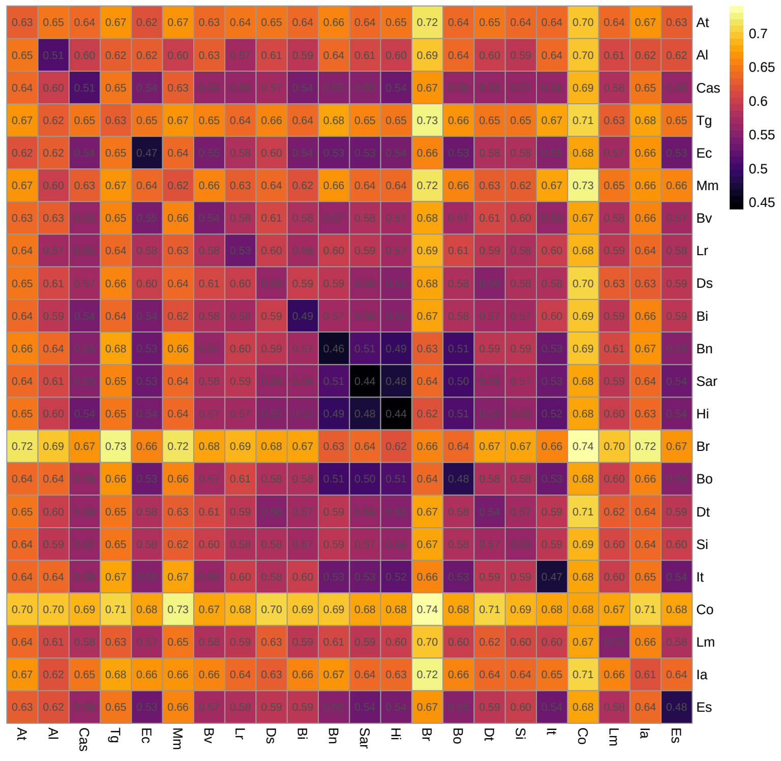
16S dissimilarity distance
