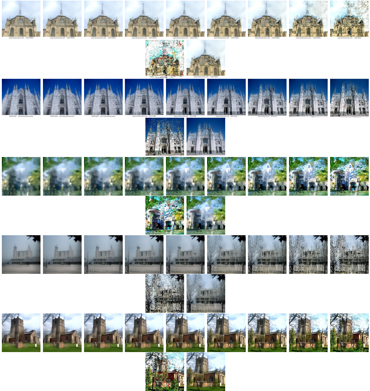
Figure 31: DDPM sampling with 20 steps. For each row: Columns 1-10 : only one branch with the variance scaling uniformly changing from 0.05 to 1.95. Column 11 : image sampled with our method.
