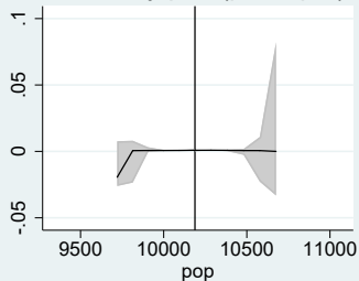
rddensity plot (p=2, q=3)
