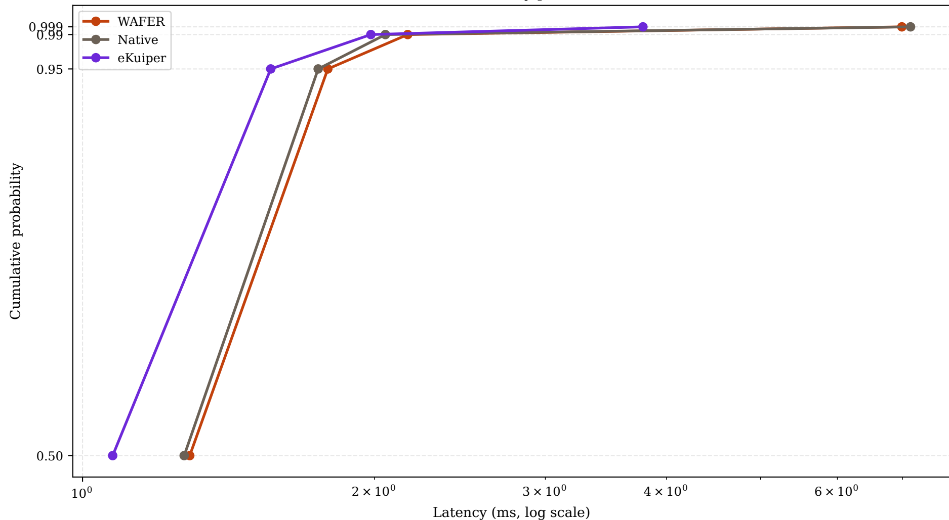
Figure 1: Latency CDF comparison (shakedown-macos) CDF reconstructed from summary percentiles: 50, 95, 99, 99.9
