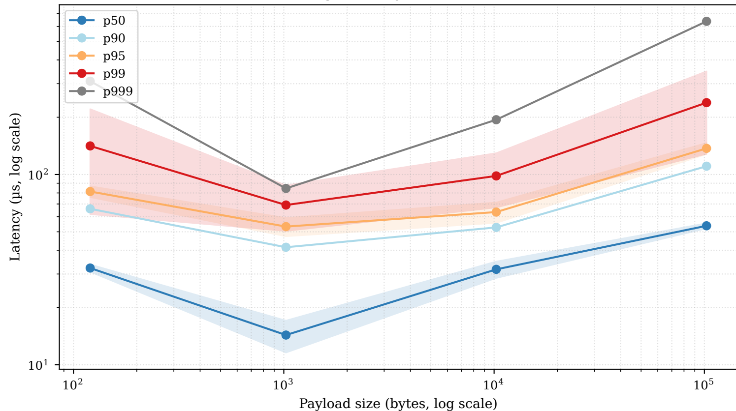
E-Perf-4 per-hop overhead — shakedown-macos-2026-07-21T20-08-17Z pipeline-c-passthrough × 4 payload sizes (shaded = 95% CI)
